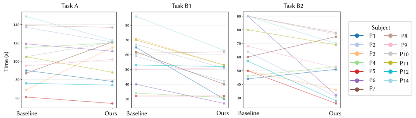
Figure 20: Visualization of paired differences for each participant.
