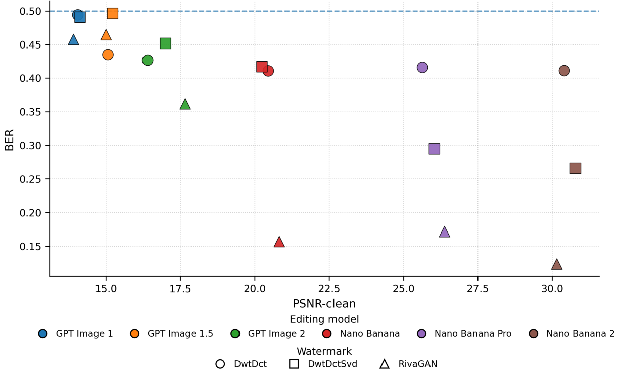
Figure 3: Victim BER versus clean-reference PSNR. Marker shape denotes the watermark scheme. The dashed line marks random binary recovery.
