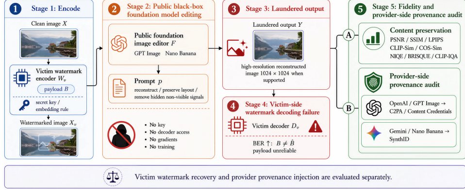
Figure 1: Threat model and evaluation for single-prompt watermark laundering through a public black-box foundation image editor. An attacker submits a watermarked image and a single reconstruction prompt without access to the victim decoder, embedding key, model parameters, gradients, or detector feedback. The reconstructed output is evaluated separately for victim-payload recoverability and content preservation.
