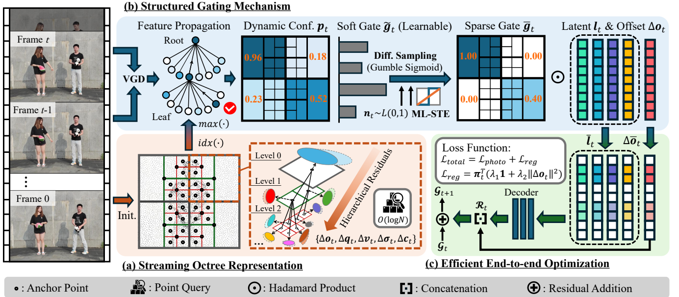
Fig. 3. Overview of the proposed S 2 GS framework. (a) The streaming octree representation is initialized using root Gaussian primitives from the first frame and subsequently represents FVVs with multi-resolution grids, enabling hierarchical allocation of Gaussian residuals and efficient point queries for FVV streaming. (b) A structured gating mechanism is introduced to induce sparse Gaussian residual updates through hierarchical feature propagation, differentiable sampling with Gumbel-Sigmoid, and multi-level (ML) discretization using a straight-through estimator (STE). (c) A sparse regularization loss is incorporated to enable efficient end-to-end optimization of structured gates and sparse residual updates.
