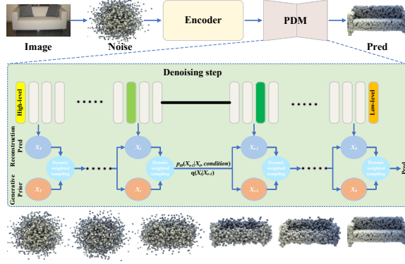
Fig. 1: Schematic Illustration of Our PDM. PDM reconstructs original point clouds from noisy inputs. An Encoder extracts image-conditioned features from a single-view image. At each Denoising step, a Dynamic Weighted Sampling (DWS) strategy fuses two representations: the reconstruction prediction and generative prior. Guided by these projected features and DWS, the network learns richer hierarchical geometric priors to progressively generate the final prediction.
