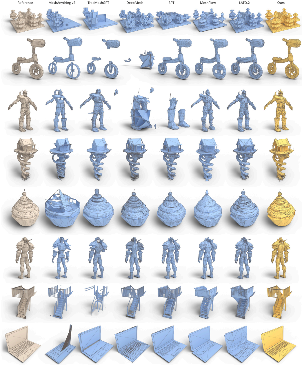
Figure 3: Qualitative comparison on Objaverse and Toys4K. References are in clay, baselines in blue and MeshCarve in amber; all outputs are shown as generated with wireframes. Zoom in for better view.
