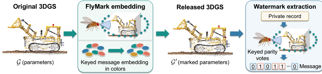
Figure 1: FLYMARK writes a message where a fly looks. A virtual observer carries the connectome’s photoreceptor directions around the scene, and each direction reads an opacity-weighted cone of Gaussians. Embedding perturbs only the stored degree-zero colors, so the marked render \mathcal{G}' is high visual fidelity from \mathcal{G} ; extraction replays the same orbit readout with the key. The fly, orbit, and bit glyphs are schematic.
