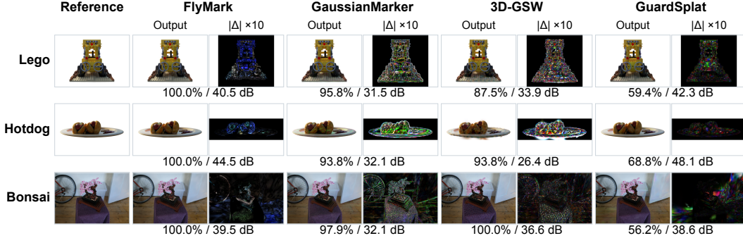
Figure 3: Registered-view qualitative comparison on Lego, Hotdog, and Bonsai. Every method is shown as an equal-size output/difference pair, where the right panel is the 10\times absolute RGB difference from the matched reference under a shared display transform. In the one-line annotation beneath each marked pair, the value before the slash is key-17 bit accuracy (%) and the value after it is direct PSNR (dB) for the displayed frame. Each row uses identical cameras and crops across methods, and Bonsai uses the third registered view (frame 29). Tables 1 and 2 report aggregate recovery and fidelity; Appendix H shows all three registered views.
