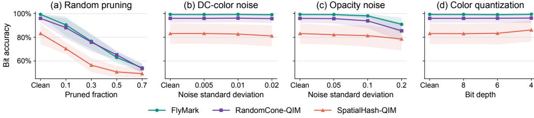
Figure 4: Bit accuracy under four representative model-attack families. Lines are scene-first means over ten scenes and three watermark keys, and shaded regions show hierarchical-bootstrap uncertainty. The clean point is repeated as severity zero.
