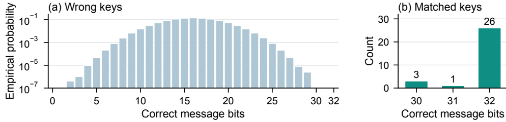
Figure 5: Wrong-key calibration. The left panel plots empirical probability by correct message bits over five million wrong-key trials (logarithmic vertical axis); the right panel counts clean matched-key scores across 30 scene/key cells. The preselected ownership cutoff is 30 correct bits.
