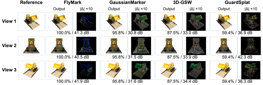
Figure 7: Lego at registered frames 40, 100, and 159. For FLYMARK, GaussianMarker, 3D-GSW, and GuardSplat, the equal-size panel to the right of each output shows its 10\times absolute RGB difference from the matched reference. The one-line values are key-17 bit accuracy (%) / direct PSNR (dB), with PSNR evaluated at the displayed frame.
