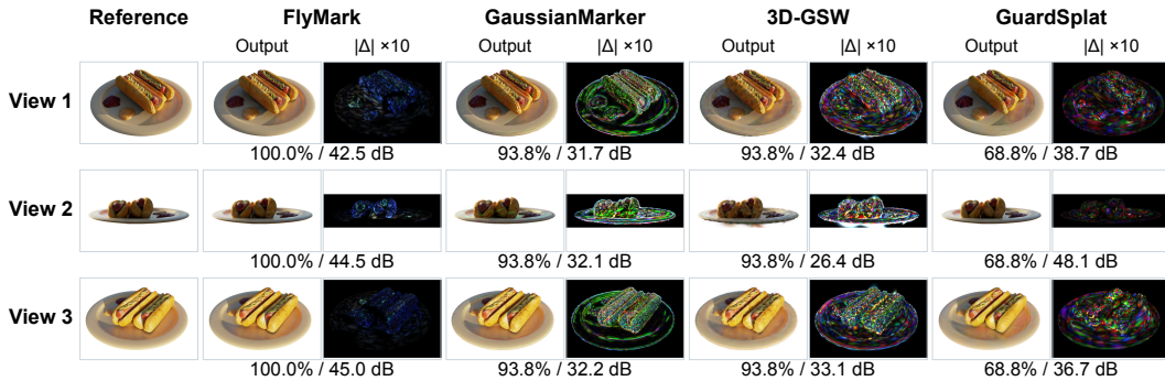
Figure 8: Hotdog at registered frames 40, 100, and 159. For FLYMARK, GaussianMarker, 3D-GSW, and GuardSplat, the equal-size panel to the right of each output shows its 10\times absolute RGB difference from the matched reference. The one-line values are key-17 bit accuracy (%) / direct PSNR (dB), with PSNR evaluated at the displayed frame.
