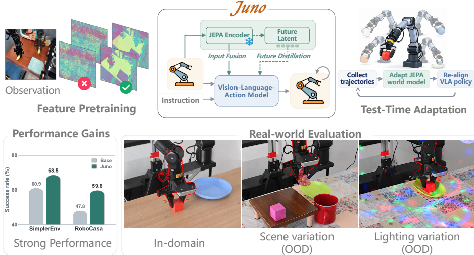
Figure 1: We present Juno, a unified framework that makes predictive latents useful across the vision-language-action (VLA) lifecycle. Juno integrates control-aligned JEPA pretraining, visual feature fusion and decoupled future-latent distillation, and dynamics-first test-time adaptation that updates the world model before re-aligning the policy. It improves performance on SimplerEnv and RoboCasa and supports robust real-world manipulation under distribution shifts.
