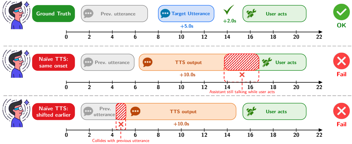
Figure 4: Why naive TTS synthesis on video-text dialog data is insufficient. The ground truth instructor (top) times utterances to finish before the user’s next action. Naive TTS (middle) generates longer speech that overlaps with the user’s action. Shifting the onset earlier (bottom) avoids the action overlap but collides with the previous utterance and delivers guidance before the user has seen the relevant context. This motivates our choice to start from HoloAssist, where real instructor speech timing is already aligned with user actions, and to resynthesize speech with a strict duration constraint that preserves this alignment.
