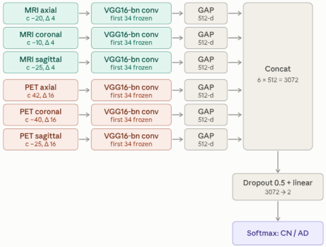
Fig. 3. Six-stream fusion architecture. Each of the six inputs (MRI and PET \times three planes) passes through an independent VGG16-BN convolutional trunk initialised from ImageNet, with the first 34 layers frozen. Global average pooling produces a 512-dimensional descriptor per stream. The six descriptors are concatenated into a 3072-dimensional vector, followed by dropout ( p = 0.5 ) and a single linear layer to two logits.
