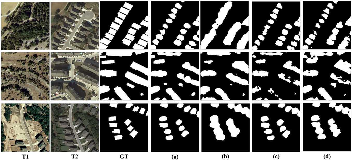
Figure 4: Qualitative ablation results. (a) Full model, (b) initial SAM pseudo-labels only, (c) initial pseudo-labels with CNN refinement (Stage I), and (d) initial pseudo-labels with self-training (Stage II).
