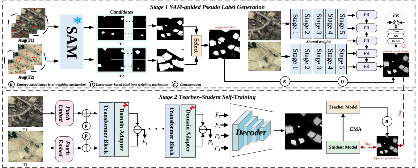
Figure 2: Overview of the proposed two-stage point-supervised change detection framework. Stage I generates and refines soft pseudo-labels from bi-temporal point supervision using SAM2, mask selection, and CNN-based refinement. Stage II further improves change detection performance through a teacher-student self-training framework with EMA update and periodic pseudo-label refresh.
