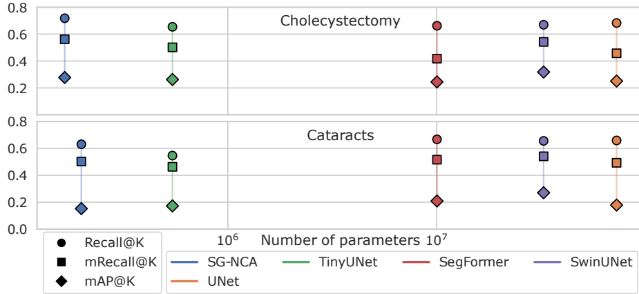
Fig. 3. Scene graph generation evaluation of semantic relationships. SG-NCA requires 55\times fewer parameters while achieving comparable performance, running on an edge device.
