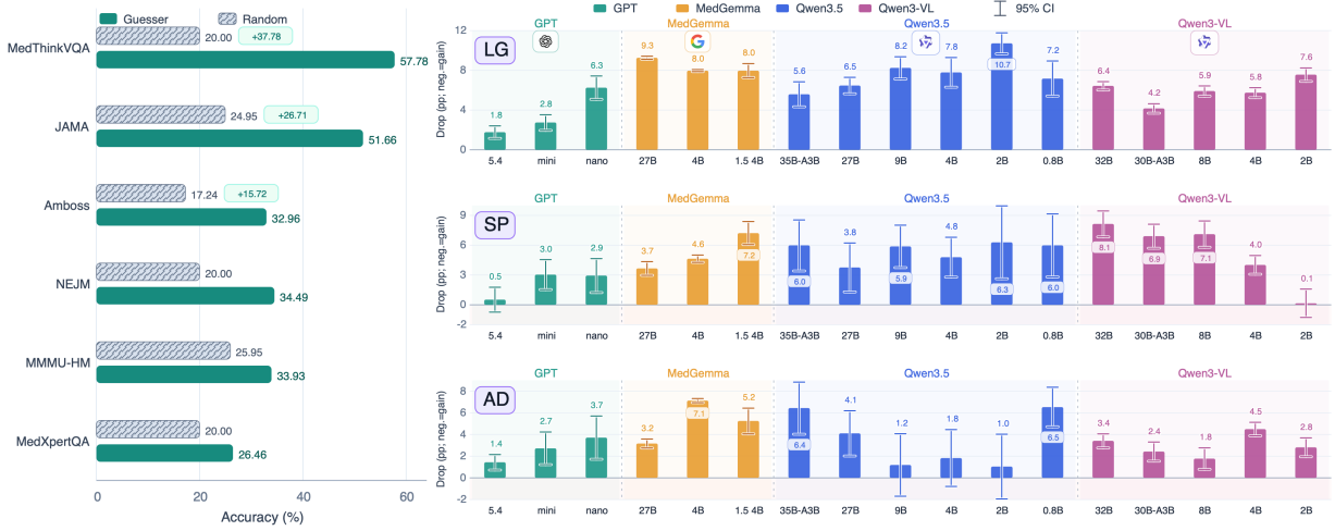
Figure 3: Option-form shortcuts create answer priors and are exposed by matched repair. A trained options-only guesser exceeds the item-level random baseline on every dataset. Matched repairs for length-gap, spatial/prepositional, and absolute/conspicuous distractor cues reduce accuracy, indicating that these option-form cues are behaviorally useful. The right-hand panels visualize positive drop magnitudes for readability; signed changes in the text and Appendix use modified minus original.
