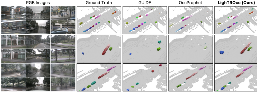
Figure 4: Qualitative comparison of GMO occupancy predictions from multi-view RGB images. LighTROcc more faithfully captures object locations and future motion, with darker colors indicating later forecasting steps.
