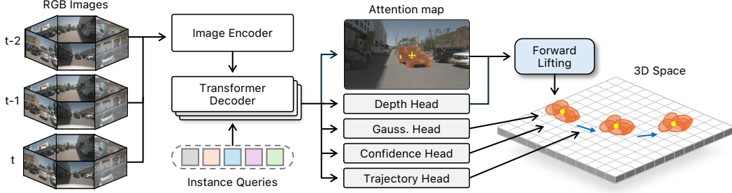
Figure 2: Overview of LighTROcc. Compact instance queries are sequentially refined through a transformer decoder using multi-view image features. Each query is localized in 3D via attention-guided forward lifting, while heads predict 3D Gaussians, confidence, and future trajectory.
