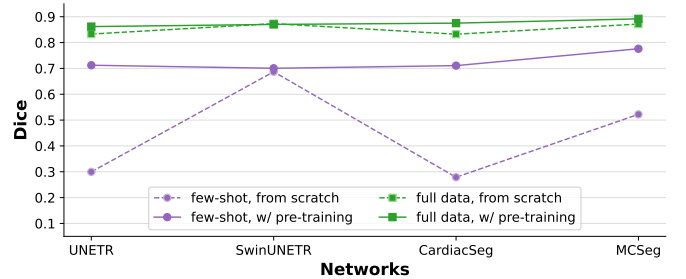
Fig. 5: Comparison of models training with and without pre-training weights under few-shot and full-data settings on ImageCHD dataset.
