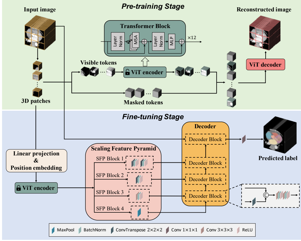
Fig. 2: The schematic overview of MCSEG. During the pre-training stage, the ViT encoder undergoes training using the MAE method. Subsequently, in the fine-tuning stage, the ViT encoder loads the pre-trained weights and freezes its parameters. The training process in this stage exclusively focuses on the SFP and the decoder.
