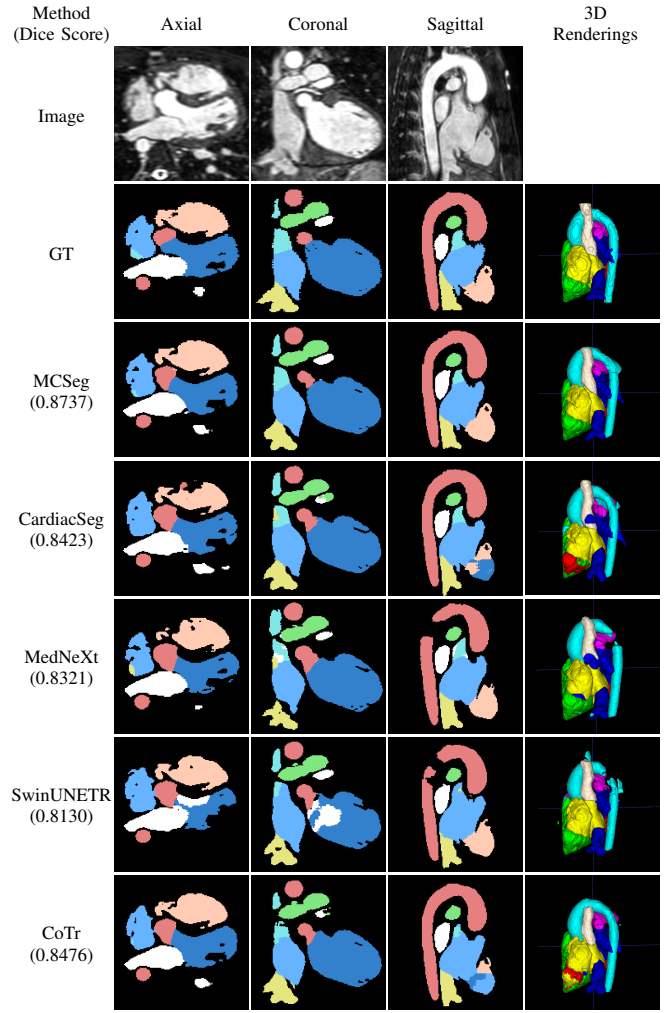
Fig. 4: Qualitative comparison for different models on image with ID “pat11” from HVSMT-2.0 dataset.
