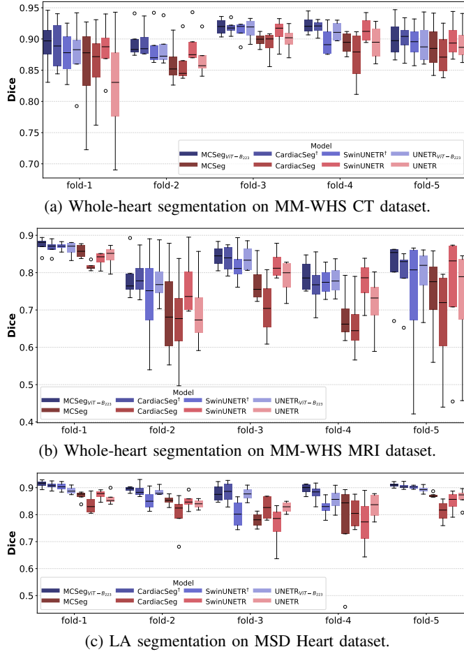
Fig. 6: Results of 5-fold cross-validation for eight models on various datasets. Models in reds are trained from scratch.
