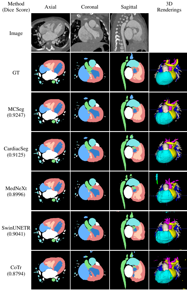
Fig. 3: Qualitative comparison for different models on image with ID “1029” from ImageCHD dataset.
