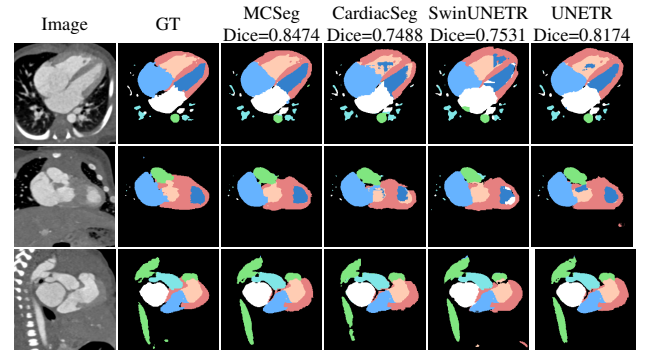
Fig. 1: Qualitative visualizations of models in few-shot experiment on image with ID “1085” from ImageCHD dataset. Results are presented in axial, coronal and sagittal views.
