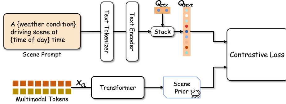
Fig. 2: The illustration of SRP module
