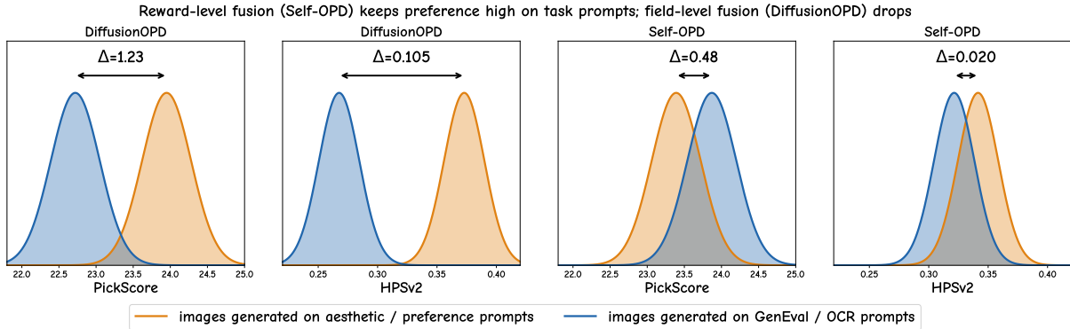
Figure 4 Field-level fusion couples preference quality to the prompt family; reward-level fusion does not. For each approach, we contrast the preference-reward distribution of images generated on aesthetic/preference prompts (orange) against that of images generated on the GenEval/OCR task prompts (blue). The distribution peaks are placed at the measured means from Tab. 2 (the “separate test set” and “same test images” columns, respectively); the spread is illustrative and only serves to visualize the shift \Delta between the two prompt families. For DiffusionOPD, the preference distribution shifts sharply when moving to the task prompts, whereas for Self-OPD, the two distributions nearly coincide.
