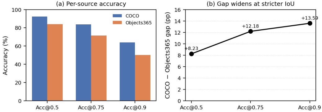
Figure 9: Source-stratified accuracy on the recombined predictions. The COCO–Objects365 gap widens as the IoU threshold tightens (+8.23, +12.18, +13.59 points), an association compatible with several localization and domain-shift explanations.
