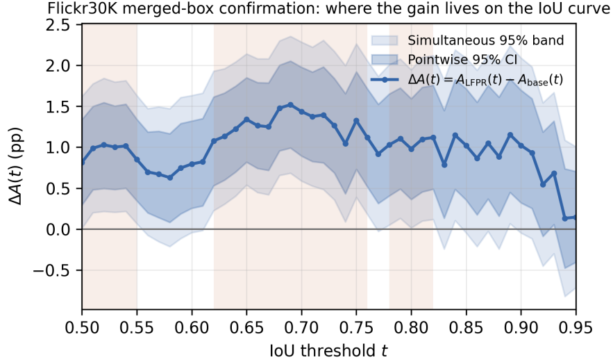
Figure 3: Treatment-minus-incumbent accuracy, \Delta A(t) = A_{\text{LFPR}}(t) - A_{\text{base}}(t) , as a function of the IoU threshold on the Flickr30K merged-box confirmation (14,481 rows, 999 images). The darker band is the pointwise 95% interval; the lighter band is the simultaneous ( \max\text{-}|T| ) 95% band used to license concentration claims without cherry-picking a threshold. Shaded vertical strips mark the grid points where the simultaneous band excludes zero. The gain is positive across nearly the entire threshold range rather than concentrated at one operating point.
