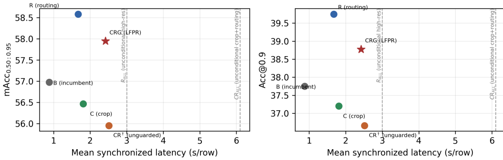
Figure 4: Accuracy-cost trade-off on the Flickr30K merged-box confirmation. Each point uses the same 14,481-row evaluation (accuracy, Table 13) and the same synchronized 512-row cost prefix on the same RTX 3090 (cost, this section); no new inference was run to build this figure. R_{ALL}/CR_{ALL} (dashed reference lines) cost 3.42 \times / 6.95 \times B ; their own matched-sample accuracy is reported in the surrounding text rather than plotted here, since it uses the smaller 512-row sample rather than the full population the other five points use. On this dataset, R alone (not CRG ) is the accuracy-maximizing point on the frontier – see text.
