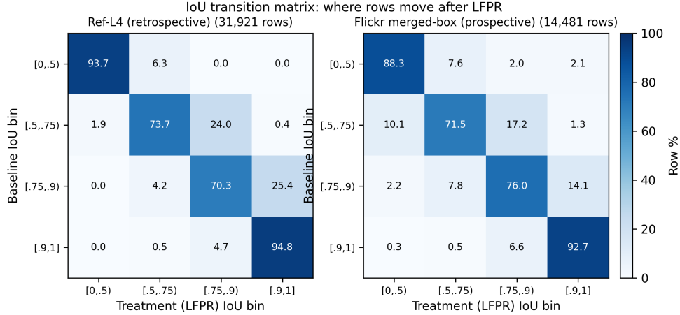
Figure 8: IoU transition matrix. Diagonal cells dominate on both datasets (70–95% of rows stay in their baseline bin), consistent with LFPR changing a minority of predictions (Section E.7). The two off-diagonal cells of most interest: strict-IoU harm, [\cdot 9, 1] \rightarrow [\cdot 75, \cdot 9] , affects 4.7% of Ref-L4’s near-perfect rows (894/18,847) and 6.6% of Flickr’s (359/5,467) – a real, nontrivial cost, not a rounding artifact, consistent with the guard-versus-Acc@0.9 trade reported throughout this paper. Genuine boundary refinement, [\cdot 5, \cdot 75] \rightarrow [\cdot 9, 1] , is comparatively rare on both datasets (0.4% Ref-L4, 1.3% Flickr); most of LFPR’s gain instead comes from the larger [\cdot 75, \cdot 9] \rightarrow [\cdot 9, 1] cell (25.4% Ref-L4, 14.1% Flickr), i.e. rows that were already close and get pushed over the strict threshold, not rows recovered from a coarse miss.
