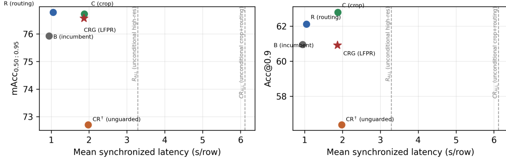
Figure 6: Accuracy-cost trade-off on the RefCOCO-family transfer split. Each point uses the same 30,969-row evaluation (accuracy, Table 11) and the same synchronized 512-row cost prefix on the same RTX 3090 (latency, Table 18); no new inference was run to build this figure. CRG (LFPR, starred) costs 1.865s/row against B ’s 0.945s/row, a 1.97\times increase – consistent with the paper’s “approximately doubles inference latency” characterization, since every admitted row pays one crop pass and router-flagged rows may pay an additional high-resolution pass. The two unconditional controls this cycle added, R_{ALL} and CR_{ALL} (dashed reference lines), cost 3.48\times and 6.48\times B respectively – 3.10\text{--}3.14\times more than their selective counterparts R and CR^\dagger at matched call count (Table 18) – for a policy that no longer distinguishes rows worth the extra pass from rows that are not. Their accuracy is now measured on a matched 26,488-row RefCOCO validation split (Table 19): both beat the matched B arm across all reported metrics, while R_{ALL} is stricter-threshold better than CR_{ALL} (Acc@0.9/mAcc). Because that accuracy readout is on a validation split and this figure’s selective-arm points remain on the frozen test partitions, this panel is still a cost-vs-cost picture rather than a same-split selective-versus-unconditional accuracy frontier.
