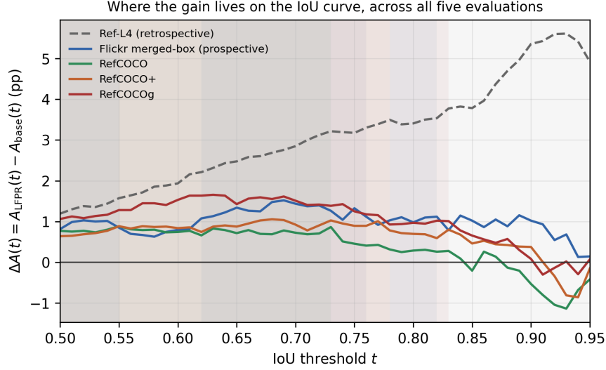
Figure 5: Treatment-minus-incumbent accuracy, \Delta A(t) , as a function of the IoU threshold, across all five evaluations, each against its own true pre-resolution incumbent B . Shaded vertical strips mark each series’ own simultaneous-band significant intervals. Ref-L4 and Flickr (retrospective and prospective evidence respectively) grow larger at strict thresholds; RefCOCO/RefCOCO+/RefCOCOg (shown individually, not pooled) stay positive through most of the range and turn negative only close to t = 0.85 – 0.92 , consistent with the deployed policy’s broad per-dataset improvement and softening strict-IoU effect reported at fixed thresholds.
