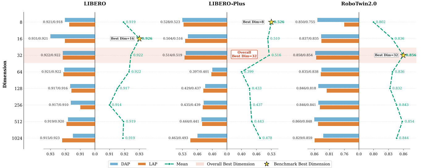
Fig. 7. Effect of latent action dimension on downstream robotic manipulation performance. We evaluate 8 latent action dimensionalities {8, 16, 32, 64, 128, 256, 512, and 1024} using LAPO with VAE regularization ( 10^{-6} ) across LIBERO, LIBERO-Plus, and RoboTwin2.0. For each benchmark, the left subplot reports the average success rates of DAP and LAP, respectively, while the right subplot reports their mean performance.
