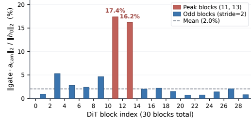
Figure 7: Per-block camera modulation amplitude. Relative camera-attention residual norm across 30 DiT blocks; red marks the two largest blocks and blue marks alternating-block injection.
