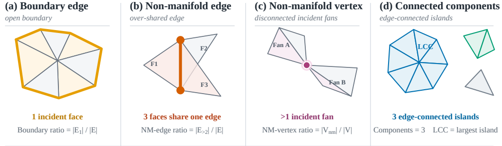
Figure 3: Topology diagnostics used in the structural audit. (a) Boundary edges have exactly one incident face. (b) Non-manifold edges are shared by more than two faces. (c) Non-manifold vertices contain multiple disconnected incident-face fans around the same vertex. (d) Edge-connected components are maximal face sets joined through complete shared edges; LCC denotes the largest component.
