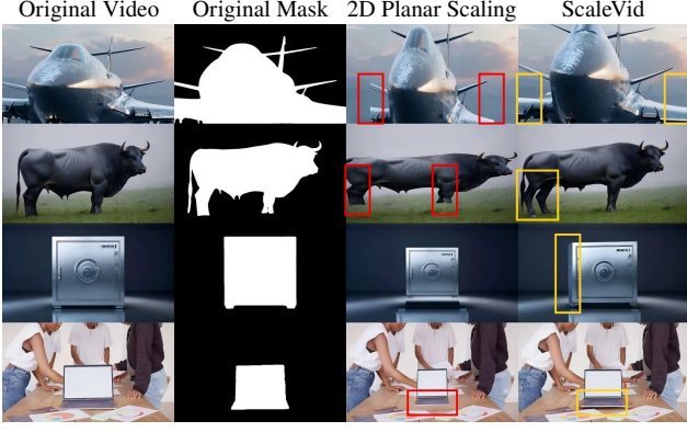
Figure 4: Visual comparison between 2D scaling & ScaleVid.
