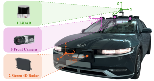
Fig. 6. Sensor configuration for the stereo 4D Radar dataset.
