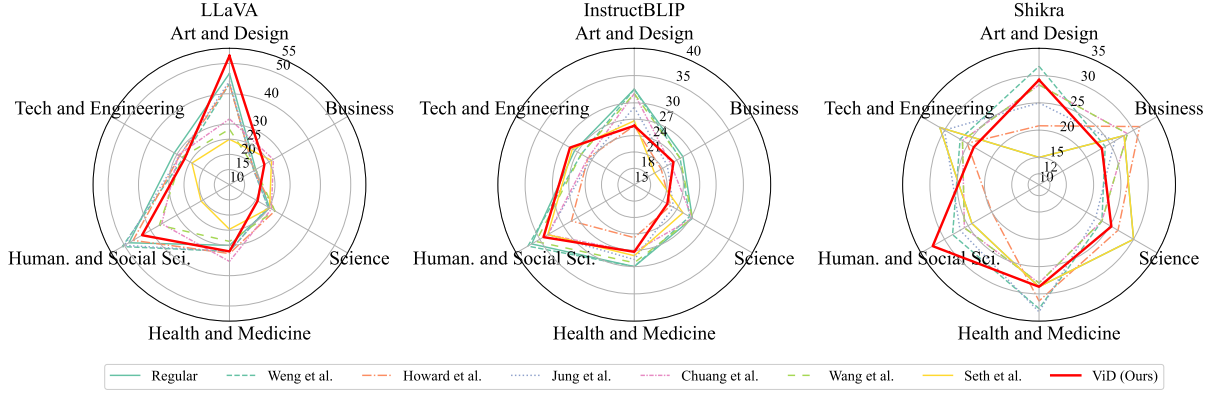
Figure 3: Radar chart of accuracy distributions across academic domains in the MMMU benchmark.
