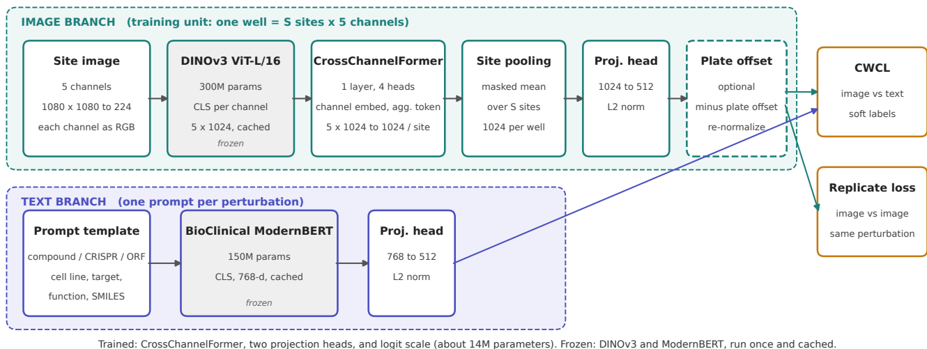
Fig. 1. Overview of MorphoCLIP. A frozen DINOv3 encoder processes each fluorescence channel separately, and the CrossChannelFormer combines the resulting tokens. Site representations are averaged into a well representation and projected into the shared embedding space. A frozen BioClinical ModernBERT encodes the perturbation prompt, followed by a trainable text projection. Optional plate correction is applied to the image embedding before the training losses.
