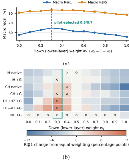
Fig. 7. Channel-weight sensitivity over 11 pairs. (a) Macro Recall@1/5; dashed: IH+G-pilot selection ( w_l, w_h ) = (0.3, 0.7). (b) Recall@1 change from equal weighting for the seven Table II conditions; circles mark row maxima and the outline marks the selected pair.
