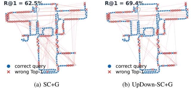
Fig. 5. Top-1 retrievals for all 320 eligible IH queries (shared +G protocol): blue circles correct, red crosses failures linked to their selected keyframes, gray trajectories.
