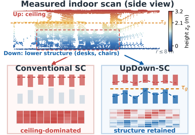
Fig. 1. Why maximum-height SC loses indoor structure. Top: a gravity-canonicalized side view of one measured 0.1-s indoor query, colored by height. The dashed line marks the map split \tau_g ; the display omits far and above-ceiling returns. Where lower and overhead structure share a polar cell, SC keeps only the upper maximum. UpDown-SC keeps both envelopes. Lower panels are schematics, not measured performance.
