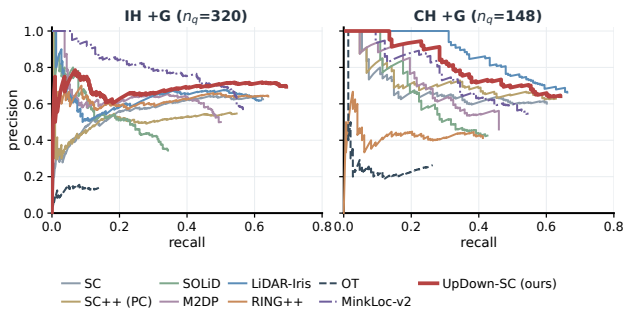
Fig. 6. Top-1 acceptance precision-recall under the shared gravity-canonicalized protocol. UpDown-SC attains the best F1max/AUPR on IH (0.696/0.475, vs. 0.643/0.398 for RING++) and the second-best on CH (0.644/0.530) behind LiDAR Iris (0.671/0.587) at roughly 40× its query latency. BTC lacks a comparable scalar confidence.
