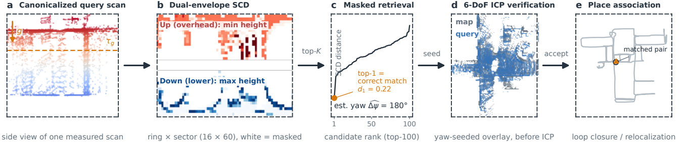
Fig. 2. End-to-end pipeline on one measured IH query from the 2 m evaluation. The shared map/query front end canonicalizes gravity and builds the dual-envelope SCD. Mask-aware retrieval returns ranked place and yaw hypotheses (here \hat{\Delta\psi} = 180^\circ ), and point-to-map ICP verifies each 6-DoF seed. Panel (d) overlays the query on the retrieved keyframe using only the descriptor seed, before ICP. Retrieval metrics are measured before ICP.
