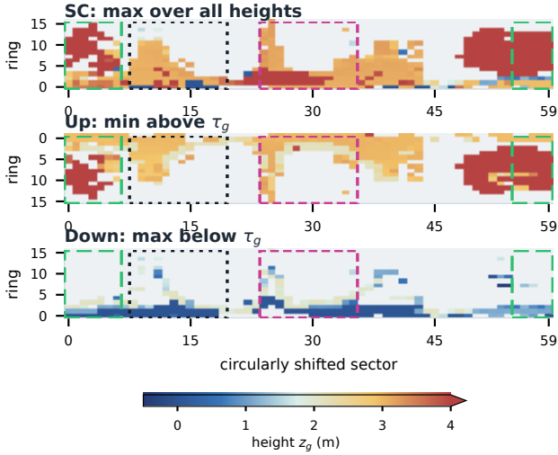
Fig. 4. Rectangular SC-style feature maps of the same query as Fig. 3, sharing one 16 \times 60 grid, color scale, and circular shift (Up drawn with near rings at the top, as in Fig. 2). Up retains SC’s overhead support (431 cells, 92.3%); Down restores all 197 lower/middle observations hidden by SC’s full-height maximum. Data-selected 12-sector windows mark three advantages: magenta, the densest mixed-cell region (59 cells); green dashed, 49 overhead cells whose stored maximum and visible underside differ by a median 2.2 m (kept only by Up); black dotted, lower structure spreading 0.90 m where overhead pins SC’s spread to 0.35 m. No value is interpolated or edited.
