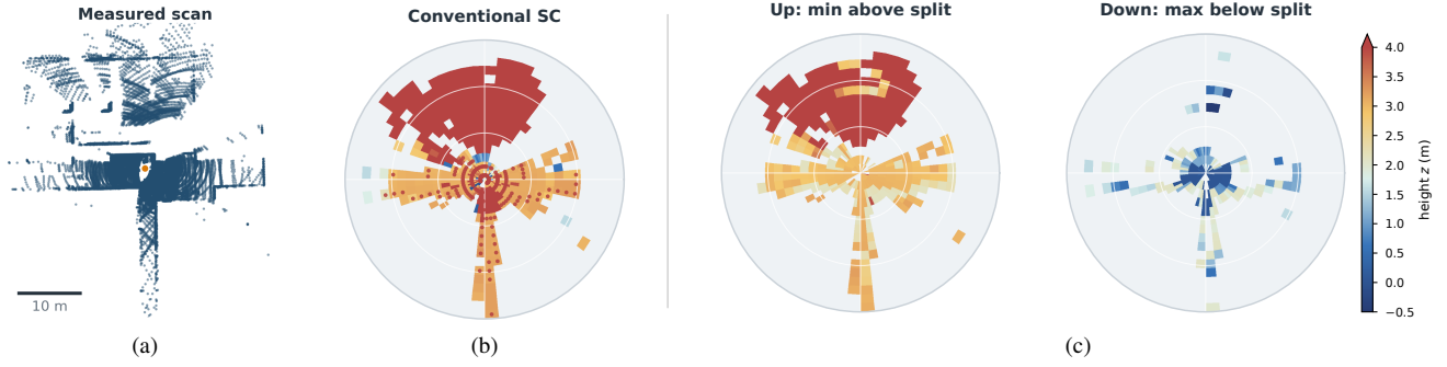
Fig. 3. One measured query shown at a common gravity-canonicalized reference. (a) White-background top view with a display-only crop of sparse range-boundary returns; all valid points still enter the descriptor, and the orange marker is its origin. (b) Conventional SC is dominated by overhead maxima in 431 of 467 occupied cells; 197 of these cells also contain lower/middle returns. (c) Up retains the overhead layer and Down separately retains the lower/middle layer. Descriptor heights share a color scale capped at 4.0 m, with the triangular tip denoting larger values.
