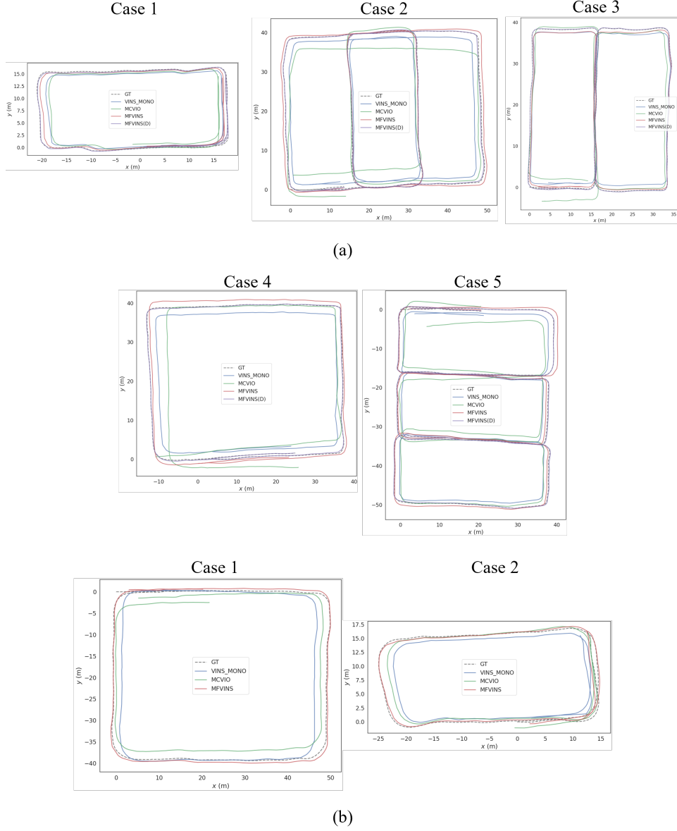
Figure 9: (a) and (b) show qualitative results of trajectory estimation on the DRIVING and OCCLUSION sequences, respectively. The dashed line denotes the ground-truth trajectory. The blue represents VINS-Mono, green represents MCVIO, red represents MFVINS, and purple represents MFVINS(D).
