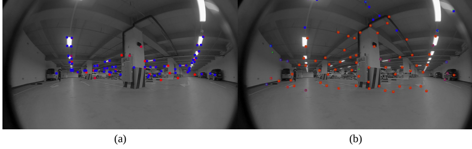
Figure 2: An example of feature detection and tracking (Blue: detected, Red: tracked, Green: predicted features) (a) MCVIO using VPI-Harris, (b) proposed method.
