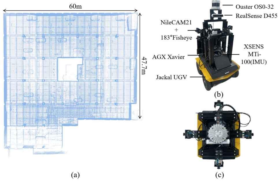
Figure 7: (a) 3D point cloud map of underground parking lot where experiments conducted; (b), (c) Side and top views of the mobile robot platform equipped with multiple sensors, respectively.
