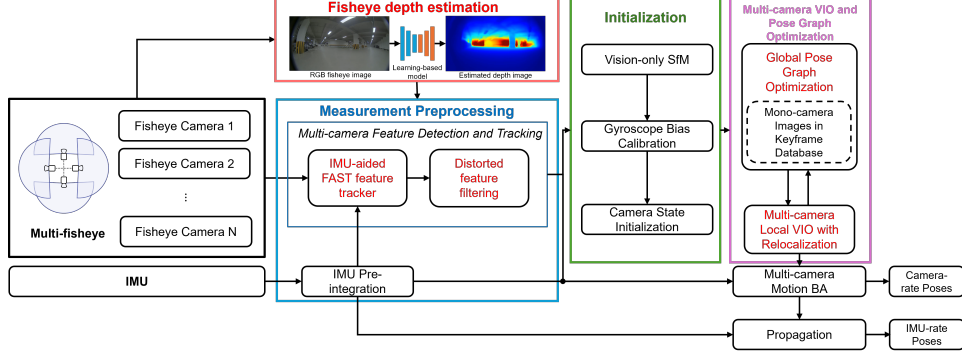
Figure 1: Framework of the proposed Multiple Fisheye Visual Inertial Systems (MFVINS). The upgraded modules are highlighted in red.
