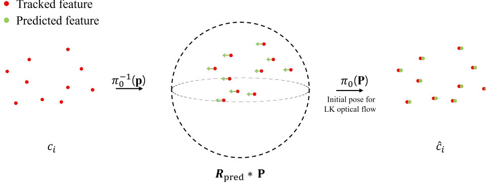
Figure 3: Predicting feature point locations using a rotation matrix
