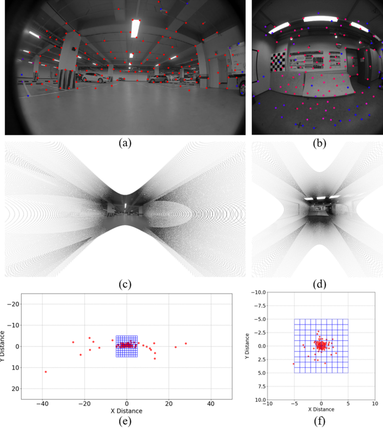
Figure 4: Comparison of feature distributions on the normalized image plane between TUM VI and our 16:9 fisheye dataset. (a), (b): Tracked feature points on the raw fisheye images. (c), (d): Distortion-corrected fisheye images. (e), (f): Distribution of tracked features projected onto the normalized plane.
