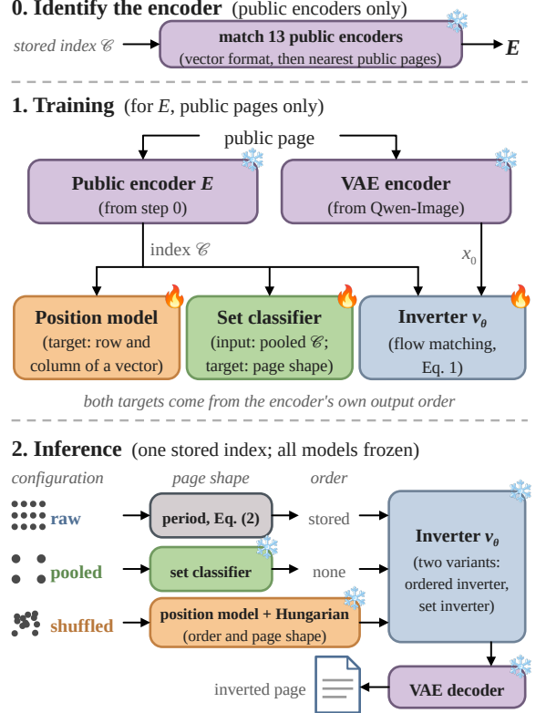
Figure 2: The three steps of the attack. Flames: models the attacker trains for an encoder E ; snowflakes: frozen models, which at inference include all of them. Step 0 identifies E from the stored index with public encoders alone (§4.2); step 1 trains models for E on public pages; in step 2, each row shows, per storage configuration, where the page shape and the order come from. The inverter uses its ordered variant when the order is known and its set variant otherwise (§4.1).
