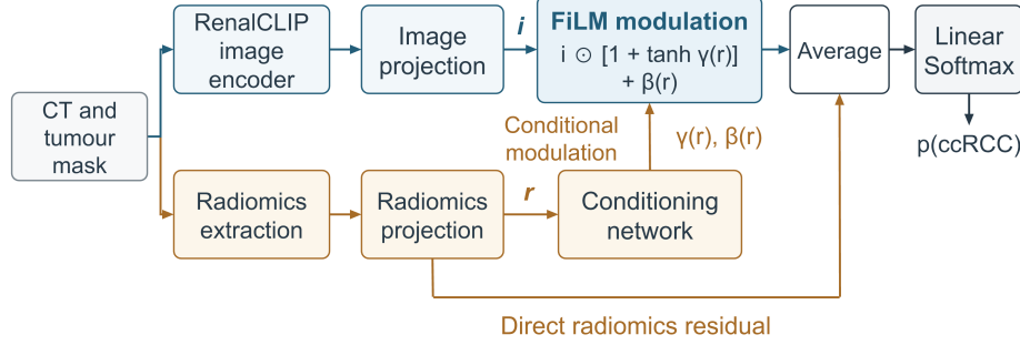
Fig. 1. Radiomics-conditioned residual FiLM. Radiomics guides the affine transformation of image features and contributes directly to the fused representation. The image encoder is fixed while the projections, conditioning network, and classifier are learned.
