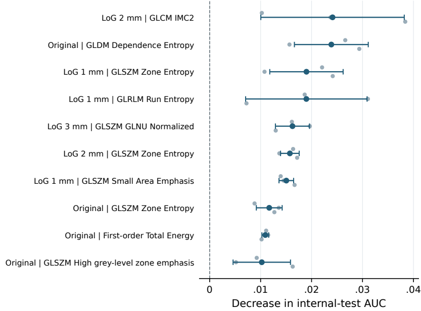
Fig. 2. The ten radiomics features with the largest mean AUC decrease under permutation. Blue markers and bars show mean \pm SD across runs, and grey markers show individual-run means over 50 permutations. GLCM, GLRLM, GLSZM, and GLDM denote co-occurrence, run-length, size-zone, and dependence matrices. GLNU denotes grey-level nonuniformity.
