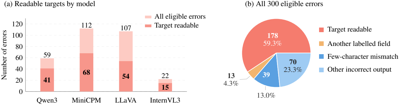
Figure 3. Target readability in 300 configuration-induced errors. (a) Bars show total errors and the subset with complete target transcription through guided reading for each model. (b) The pie shows the overall distribution; remaining cases are classified by outputs under a common reading prompt.
