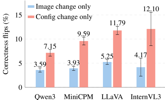
Figure 2. Bars show four-task mean correctness-flip rates when changing only the image or configuration; error bars indicate 95% confidence intervals clustered by source.
