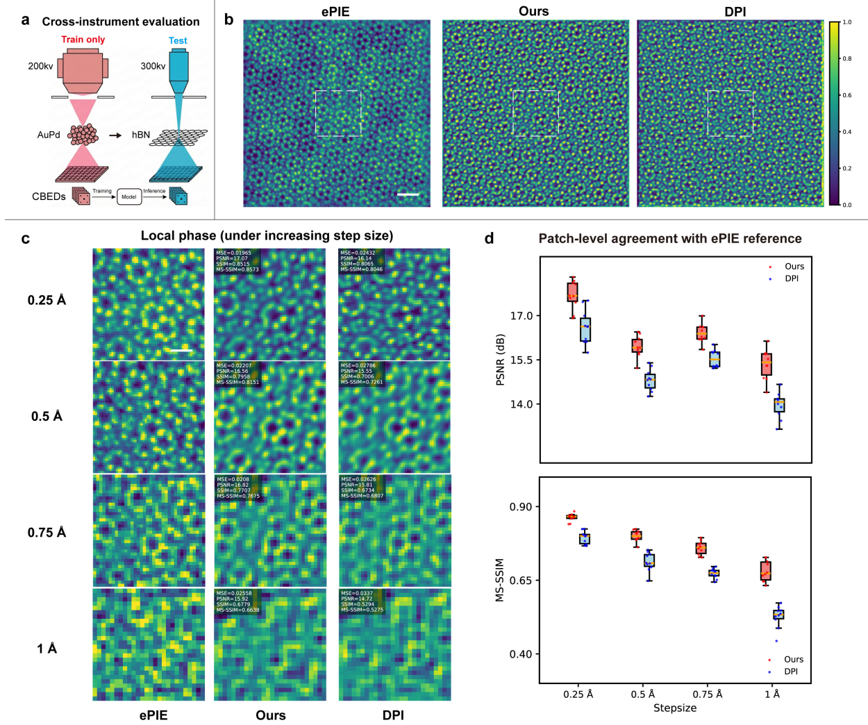
Fig. 5 | Cross-instrument zero-shot transfer and sparse-sampling robustness.
