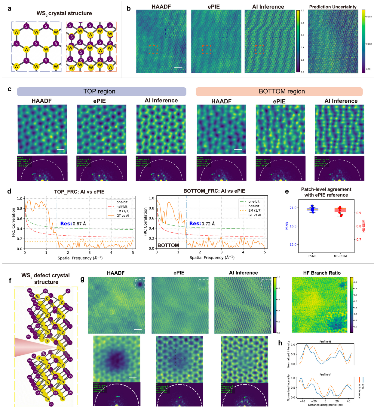
Fig. 3 | Cross-material zero-shot transfer from AuPd to WS_2 .
