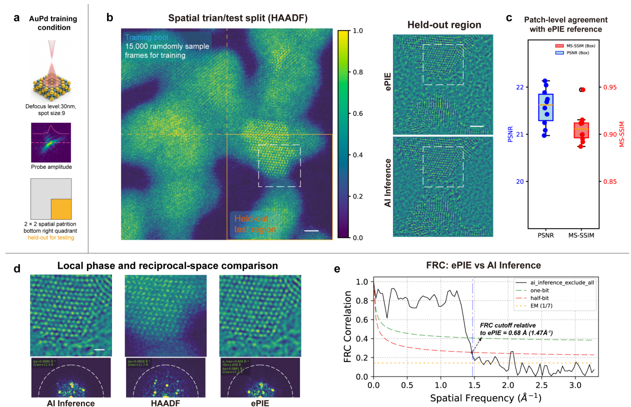
Fig. 2 | Spatial hold-out validation on AuPd under matched imaging conditions.
