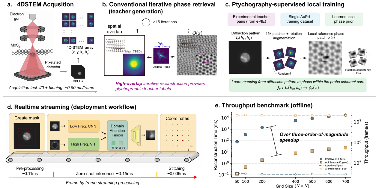
Figure 1 | Ptychography-supervised local inference for real-time electron phase imaging.
