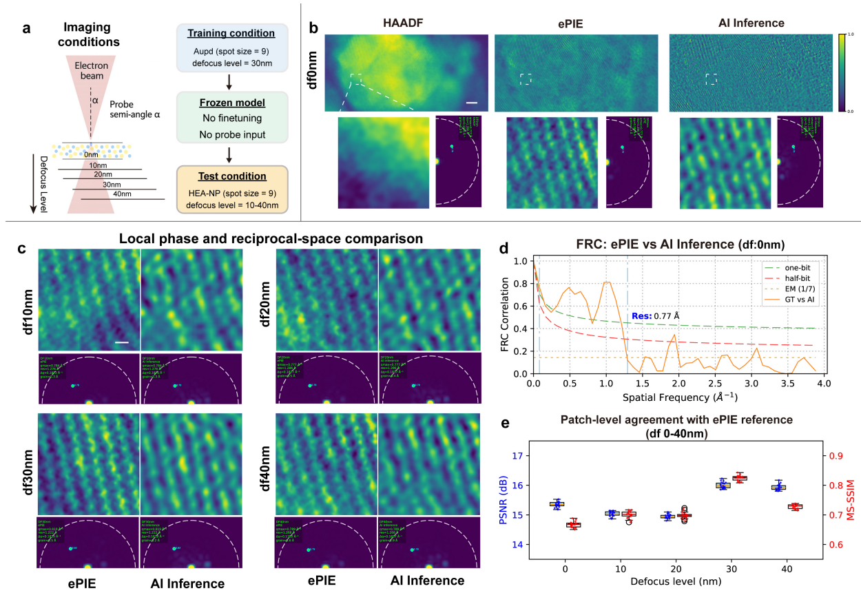
Fig. 4 | Zero-shot phase inference under continuous defocus-induced transfer-function modulation.
