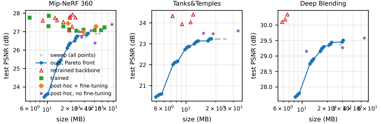
Figure 4. Rate–distortion plane on the three datasets (dataset means). Grey: every point of the sweep over pruning fraction, SH budget and codebook size of our training-free stack; blue: its Pareto front. Published methods are plotted by class (marker), from the 3DGS.zip survey and the GSICO paper; the sizes of the trained and retrained-backbone methods are not achievable without the images and are shown as context.
