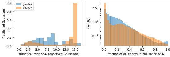
Figure 5. Spectral analysis of the observation Gram matrices of a pretrained model. Left: distribution of the numerical rank of \mathbf{A}_i . Right: fraction of the AC coefficient energy \|\mathbf{K}_i\|^2 that lies in the null space of \mathbf{A}_i , i.e. in directions no training view observed.
