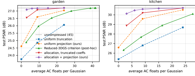
Figure 2. Rate–distortion curves (test PSNR against average AC floats per Gaussian). Uniform truncation and uniform projection have three operating points each (degrees 0, 1, 2); the post-hoc Reduced-3DGS criterion sweeps its threshold; our Lagrangian allocation sweeps the budget, with either truncated or projected coefficients.
