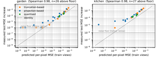
Figure 3. Predicted image-space error from the Gram metric against the measured increase of test-view MSE, over all configurations evaluated for a scene. Each point is one compressed model; hollow points lie at the noise floor of the test set.
