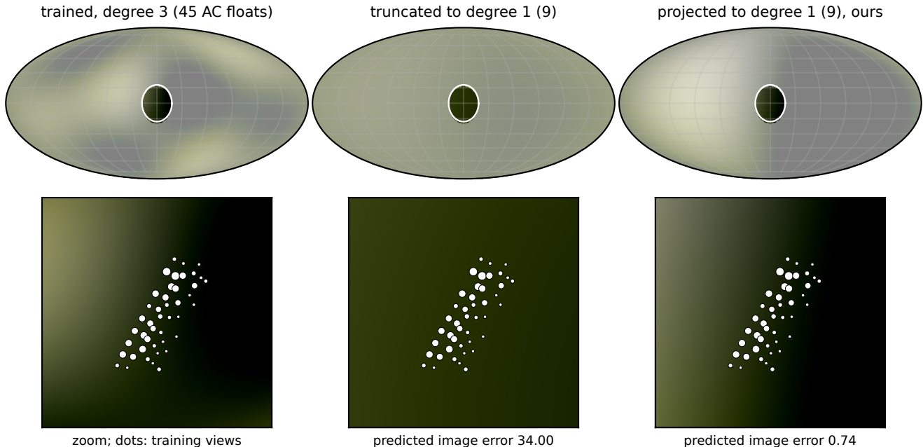
Figure 1. A trained Gaussian is only constrained where the cameras saw it. Colour function of one Gaussian of the pretrained garden model on the sphere of viewing directions (top, Mollweide projection; outside the white outline no training view observed it, shaded light) and zoomed on the observed cone (bottom; dots: the training views in which it contributed, size \propto blending-weight statistic). Truncation to degree 1 (middle) discards the bands that carry the colour gradient running through the observed cone. The closed-form observation-Gram projection to the same degree (right, Eq. (8)) reproduces the trained function where it was observed and is free elsewhere; its predicted image error is 46\times lower at identical storage.
