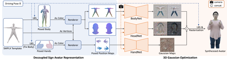
Fig. 3: Overview of sign avatar modeling pipeline. The posed vertices are taken as vertex color on the canonical SMPL-X template, and then rendered to generate posed position maps. For the hand part, we employ partial kinematic decoupling by fixing body joints, only preserving hand joint mobility. We then predict pose-dependent Gaussian maps through three specialized StyleUNet, deform the Gaussians by LBS, and render the synthesized avatar by differentiable rasterization.
