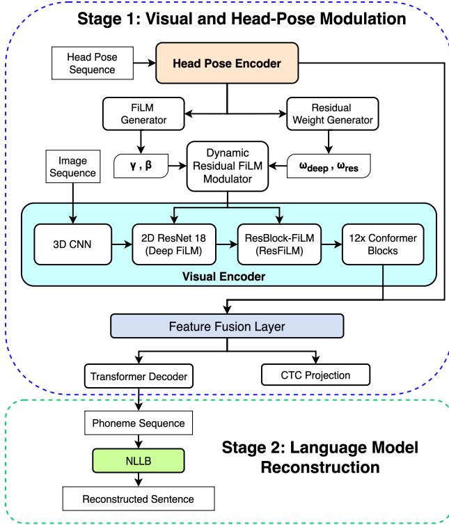
Fig. 1. Overview of the proposed architecture. Head-pose features dynamically determine the contribution of the Deep FiLM pathways at ResNet 18 Layers 3–4 and the ResFiLM pathway for pose-adaptive feature modulation.
