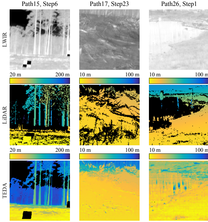
Fig. 9. Passive ranging results on additional DARPA Invisible Headlights scenes. Each column shows one acquisition group. (a) LWIR spectral-mean images. (b) LiDAR range references. (c) TEDA distance estimates. All scenes are processed with the same fixed hyperparameters, without per-scene tuning.
