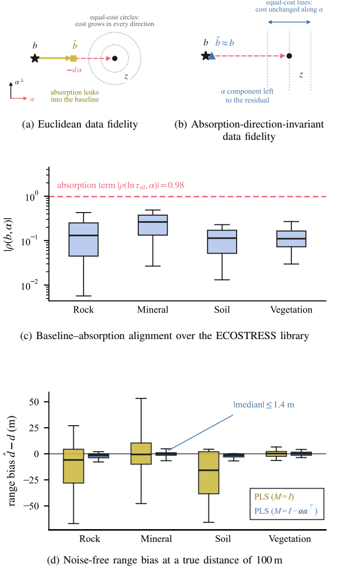
Fig. 4. Effect of excluding the absorption direction from the Stage-I data-fidelity term. (a) The Euclidean data-fidelity term allows a smooth baseline to move toward the observation along the absorption direction, causing leakage. (b) The projected data-fidelity term is invariant along this direction, so the corresponding baseline component is set by smoothness alone. (c) Absolute Pearson correlation defined in (33). Boxes summarize the correlation between the true thermal-continuum baseline and the absorption prior across emissivity spectra from the ECOSTRESS spectral library for a target 5 K colder than the air. The dashed line gives the same statistic for the sensor-domain log-transmittance, the atmospheric absorption term. (d) Noise-free range bias at 100 m under operator-consistent alignment. Both PLS estimators use the same operator-consistent distance-matching procedure; the estimator with M = I - \alpha\alpha^\top is the absorption-prior method used in Stage I of TEDA. Boxes show the interquartile range and whiskers the 5th–95th percentiles.
