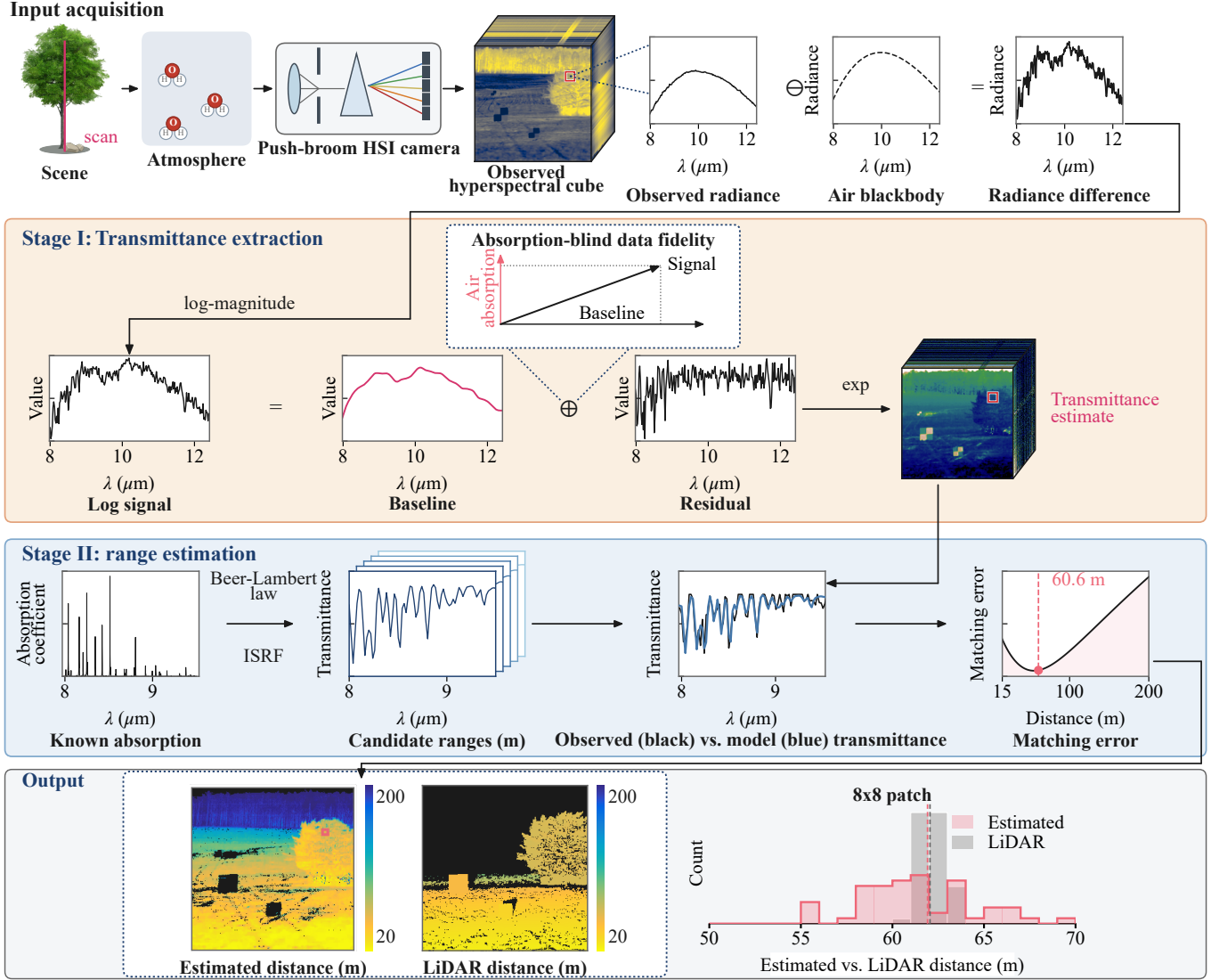
Fig. 1. Transmittance extraction and distance alignment (TEDA) for passive LWIR hyperspectral ranging. A push-broom camera scans the scene through an absorbing air path, so each measured spectrum contains range-dependent atmospheric transmittance. The red-boxed tree pixel illustrates the two-stage processing applied to every pixel. In Stage I, the known absorption structure guides the separation of atmospheric transmittance from the slowly varying thermal background. In Stage II, the extracted transmittance is aligned over the water-vapor band against model spectra that account for the sensor response throughout the distance search. The output shows the hyperspectral distance estimate alongside the LiDAR reference map; the histogram compares their distance distributions over an 8 \times 8 patch around the marked pixel. Molecular absorption is computed from HITRAN2020 for a model atmosphere with water-vapor volume mixing ratio (VMR) 0.012, temperature 289.7 K, and pressure 1010 mbar. The instrumental spectral response function (ISRF) is Gaussian with a full width at half maximum (FWHM) of 40 nm.
