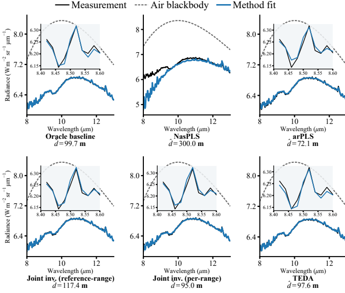
Fig. 5. Radiance-domain fits for the Rock simulation at 100 m with a target–air temperature difference of -8 K (random seed 0). Each panel compares the noisy measurement, air-blackbody radiance, and the fit from the indicated method. The Oracle baseline uses the true simulation baseline for transmittance extraction, while distance is still estimated from the noisy observation.
