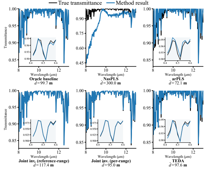
Fig. 6. Sensor-domain transmittance estimates for the Rock simulation at 100 m with a target–air temperature difference of -8 K (random seed 0). Each panel compares the true transmittance with the result from the indicated method. The Oracle baseline uses the true simulation baseline, while its distance estimate is still obtained from the noisy observation.
