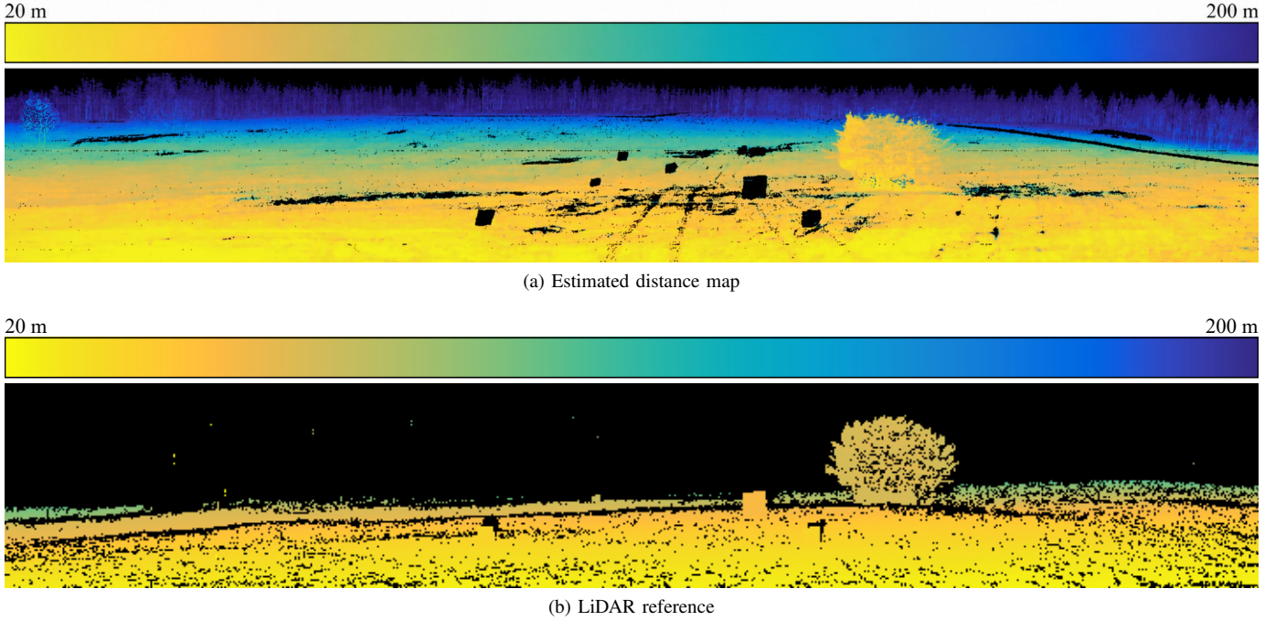
Fig. 7. Full-frame passive ranging result and LiDAR reference. (a) Distance map estimated by TEDA from the hyperspectral measurements. (b) LiDAR range map shown in the hyperspectral image coordinates for visual comparison. Both panels use the same fixed 20–200 m color scale; valid distances outside this interval are clipped to the endpoint colors. The two maps exhibit consistent near-to-far ordering across the grassland, foreground tree and background forest.
