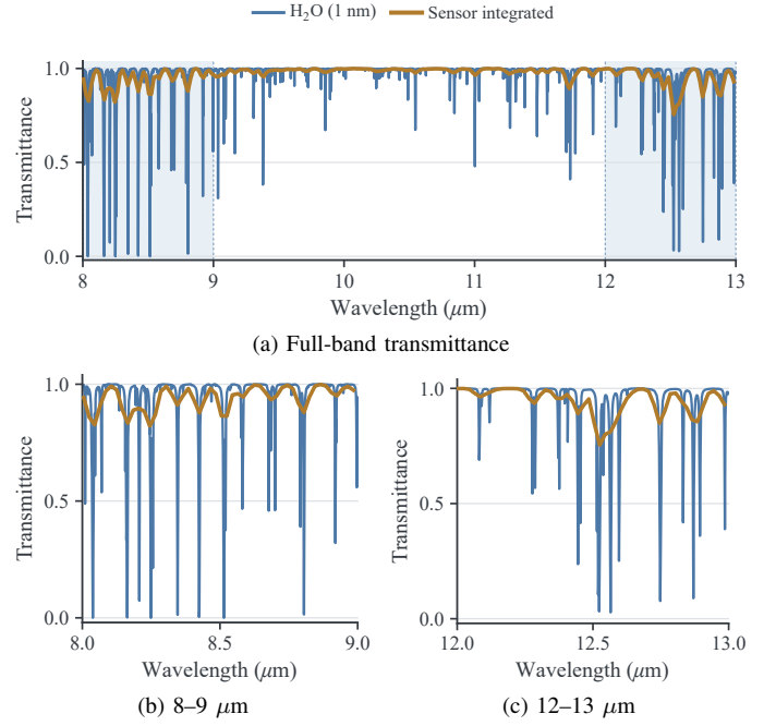
Fig. 2. Comparison of continuous-spectrum water-vapor transmittance with the transmittance after spectral-response integration. (a) Full 8–13 \mu\text{m} spectrum; the shaded intervals mark the ranges enlarged below. (b) The 8–9 \mu\text{m} absorption structure. (c) The 12–13 \mu\text{m} absorption structure. The panels compare the continuous-spectrum transmittance and the spectrally integrated result. The air temperature is 289.7 K, the pressure is 1010 mbar, the water-vapor volume mixing ratio is 0.012, and the propagation distance is 200 m. The sensor ISRF has a 40 nm full width at half maximum.
