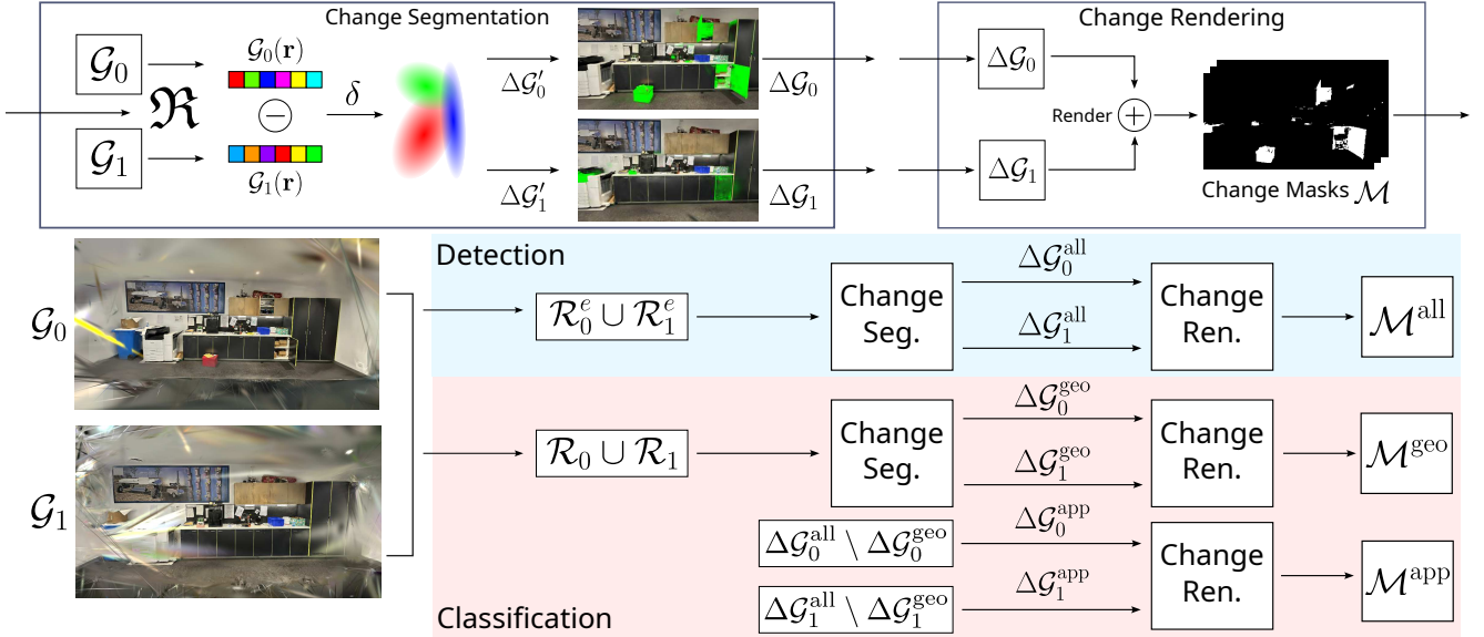
Figure 4. Our overall scene change detection and classification approach. Given instance-aware 3DGS scene representations \mathcal{G}_0 and \mathcal{G}_1 , we aggregate per-ray change scores \delta in the corresponding primitives. This yields a sparse set of anchors \Delta \mathcal{G}'_t to propagate on changed instances. For change detection, we sample edge rays \mathcal{R}^e to find changed Gaussians \Delta \mathcal{G}'_t . For change classification, we leverage PlenoCI \mathcal{R} to find geometrically changed Gaussians \Delta \mathcal{G}^{\text{geo}}_t . These explicit representations can be used to render novel change masks with disambiguation between geometric and appearance changes.
