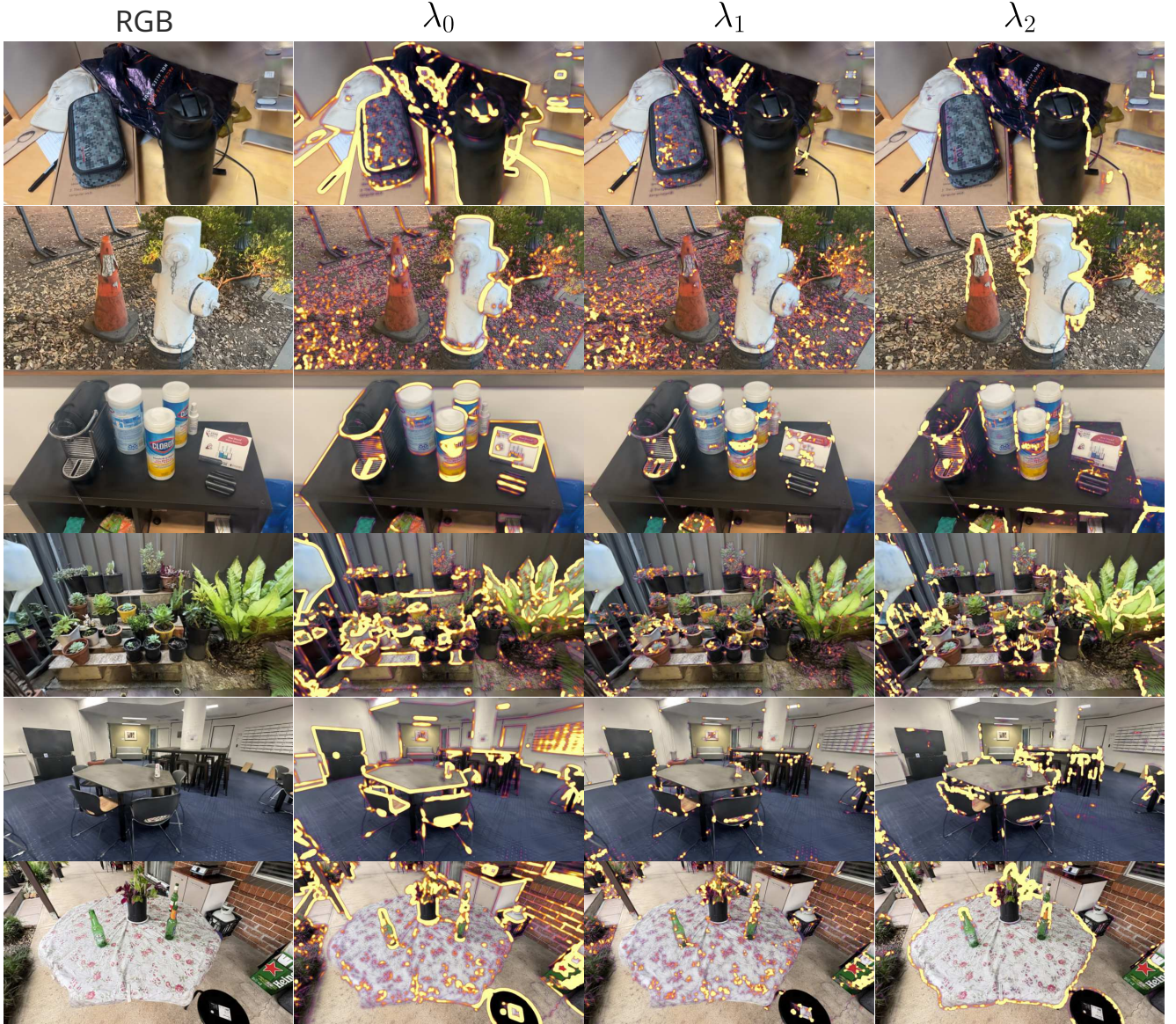
Figure 7. Pixelwise eigenvalue signals derived from the plenoptic structure tensor. Given an RGB view (column 1), we sample analytic plenoptic derivatives over a local light field to build pixelwise structure tensors M . The eigenvalues \lambda_i of M provide informative signals of scene structures, such as edges (column 2), corners (column 3) and occlusion edges as well as specular highlights (column 4).
