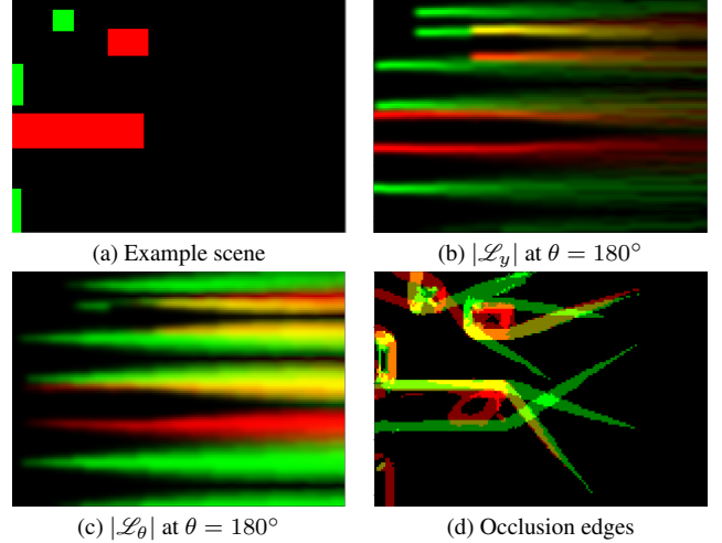
Figure 2. Example scenario in flatland to motivate our novel PlenoCI feature. Given a 2D world (Fig. 2a), we build the 3D plenoptic field \mathcal{L} and compute partial derivatives \mathcal{L}_* (Figs. 2b to 2c). These are useful signals for detecting visually complex phenomena such as occlusion edges (Fig. 2d). Brightness represents magnitude corresponding to each color channel’s plenoptic field. While we show ground truth geometry and \mathcal{L} here, this also generalizes to radiance field representations.
