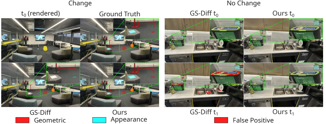
Figure 1. Given two 3DGS reconstructions from different times, our method first detects scene changes. To classify changes, we draw on view-dependent plenoptic structures encoded in our novel Plenoptic Characteristics (PlenoCI) feature. For example, we correctly detect the sheet of paper and book as changes, and classify them using PlenoCI as occlusion edge evidence (left). Our approach is robust to the inherently unconstrained nature of 3DGS representations; two independent optimizations given the same training images yield different primitive configurations. Primitive-space comparisons [22] report false positives in static scenes while our method does not (right).
