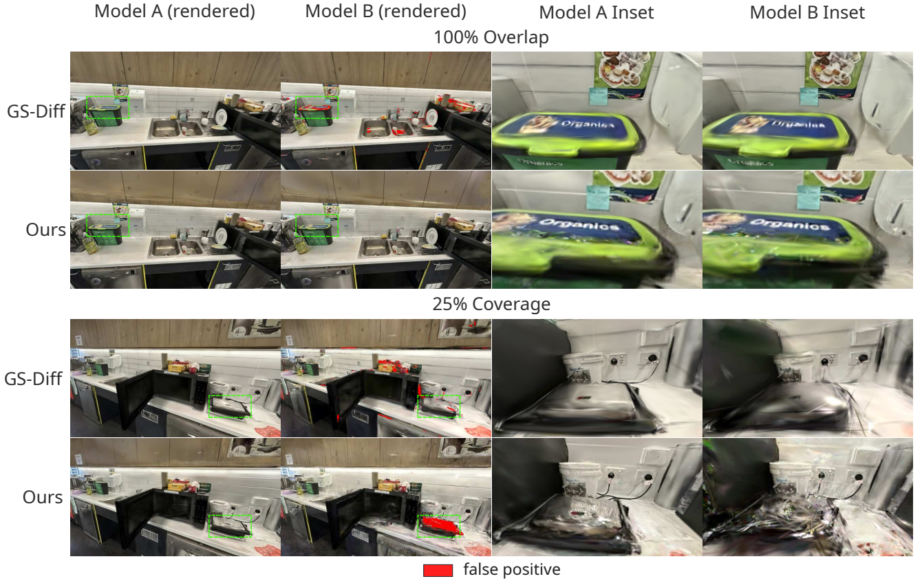
Figure 9. Comparison of independently optimized 3DGS models of the Cantina scene from PASLCD without changes. At 100% view overlap, both models receive all training views. GS-Diff [22] reports a false positive rate of 0.487% as it directly compares primitives (inset), while we correctly report no changes. At 25% view coverage, Model B receives 5 out of 20 training views. Poor reconstruction quality causes our approach to detect false positives, albeit at a lower rate than GS-Diff.
