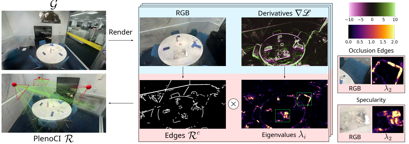
Figure 3. Our PlenoCI feature extraction pipeline. Given a 3DGS representation \mathcal{G} , we sample analytic plenoptic derivatives \nabla \mathcal{L} over a local light field to compute the structure tensor. The third eigenvalue \lambda_2 provides an informative signal for complex visual behaviors where existing features are unreliable, while ignoring Lambertian textures. We mask pixelwise \lambda_2 with an edge image (dilated for clarity) to yield PlenoCI \mathcal{R}^k from view k . Repeating this over selected views yields \mathcal{R} .
