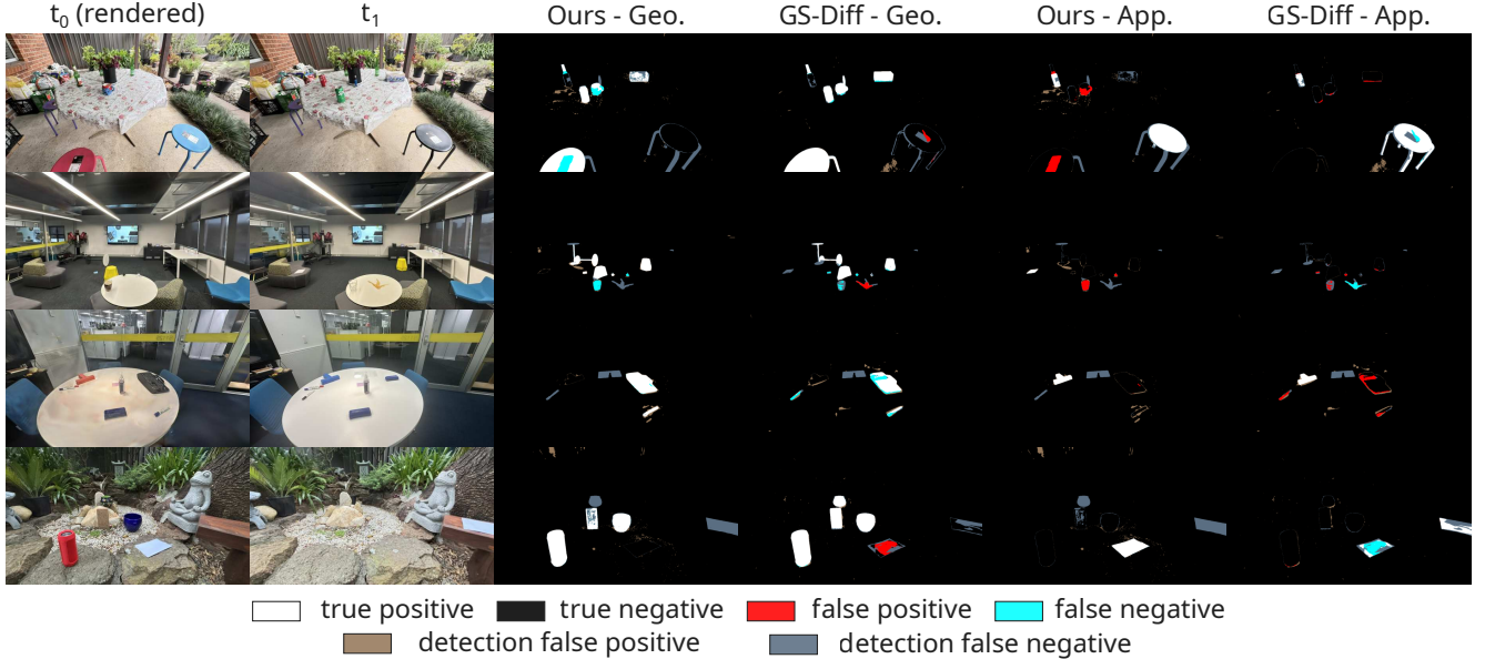
Figure 6. Qualitative change classification results for PASLCD [20]. Top to bottom: Porch, Lounge, Meeting Room, Zen. Our PlenoCI feature enables building explicit geometry and appearance-based change representations for rendering multi-class change masks.
