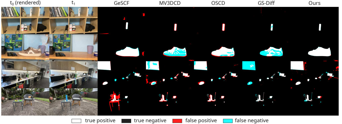
Figure 5. Qualitative comparison of binary change masks for CL-Splats [1] (rows 1–2) and PASLCD [20] (rows 3–4). Pairwise approaches such as GeSCF [35] are susceptible to spurious detections. Our instance-aware 3DGS approach outperforms all baselines on CL-Splats, and is competitive to state-of-the-art on the challenging PASLCD benchmark.
