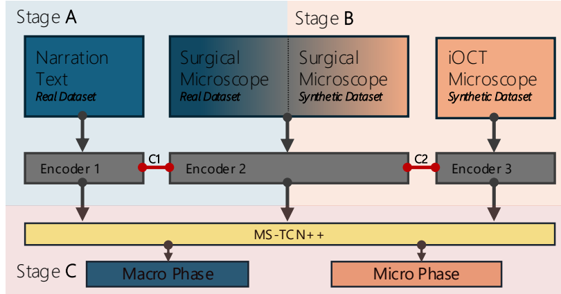
Fig. 1. Overview of the proposed framework. We use three modality-specific encoders: Encoder 1 (surgical narration), Encoder 2 (microscope view), and Encoder 3 (iOCT B-scans). Stage A: Encoder 2 is aligned to the frozen Encoder 1 via constraint C1 , bringing microscope frames and narrations into a shared domain. Stage B: with Encoder 2 now frozen, Encoder 3 is trained via constraint C2 to project iOCT B-scans into the same domain. Stage C: the resulting embeddings train the dual-head MS-TCN++ for macro- and micro-phase prediction. At inference, because semantically similar modalities occupy neighboring regions of the latent space, the MS-TCN++ predicts both macro- and micro-phases even when only the microscope view is available.
