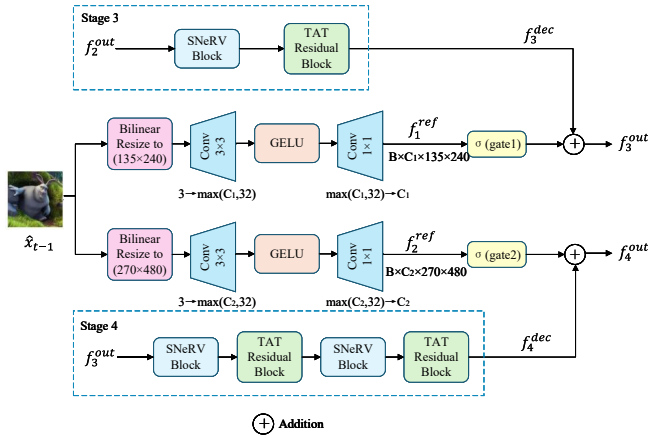
Fig. 2. Architecture of MTCF. It leverages multi-level temporal context to enhance reconstruction and suppress unreliable historical information.
