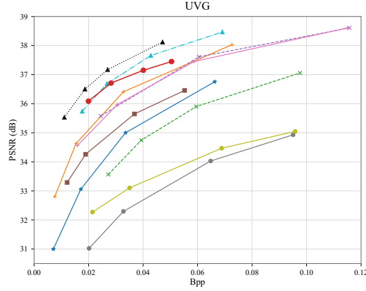
Fig. 4. Rate-distortion comparison on the UVG dataset in terms of Bpp-PSNR and Bpp-MS-SSIM.
