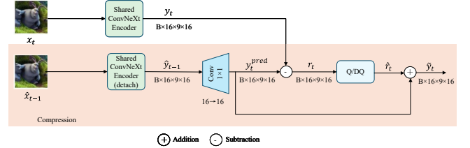
Fig. 3. Architecture of TERC. It predicts the embedding from historical context, codes the prediction residual, and thus establishes explicit frame-level predictive coding prior to quantization.
