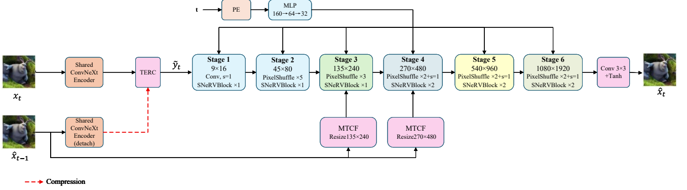
Fig. 1. Overall architecture of TCNeRV. MTCF enhances current-frame structure and texture reconstruction through multi-scale feature extraction and channel-wise gating; TERC predicts the current content embedding from historical reconstruction context and establishes an explicit temporal predictive-coding relationship among framewise content embeddings.
