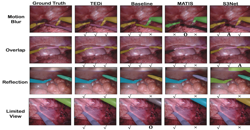
Fig. 2. Qualitative comparison of TEDi with other SOTA methods. ✓ indicates that the instrument is classified and segmented correctly. O indicates missed instance, × shows the misclassified instance and A indicates ambiguous instance.
