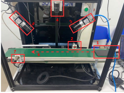
Fig. 4: Production-line prototype used for industrial evaluation: (1) test product, (2,7) photoelectric sensors, (3–5) RGB cameras, and (6) conveyor direction. The three cameras provide nominal 45°, 90°, and 135° observations.
