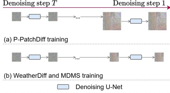
Fig. 2: Comparison of training strategy between WeatherDiff (Özdenizci and Legenstein 2023), MDMS (Shang et al. 2024) and our P-PatchDiff. (a) We gradually increase patch sizes during training to enable our denoising models to perceive more information from larger patches. (b) WeatherDiff and MDMS use a fixed patch size throughout all steps during training.
