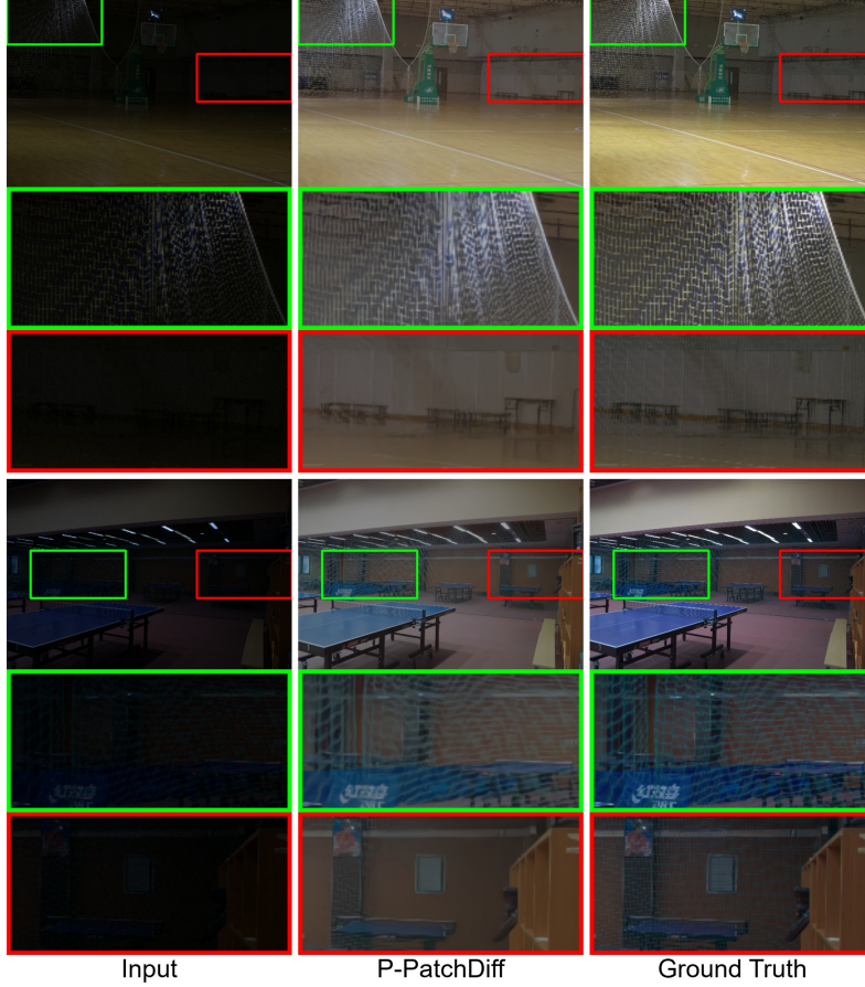
Fig. 11: Qualitative comparison of successful and failed cases, which are denoted by green and red bounding boxes, respectively. When a region is extremely dark, P-PatchDiff tends to ignore its structures (e.g., the net) entirely, rather than attempting to enhance them but failing.
