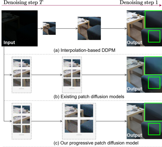
Fig. 1: Visual comparisons of recent state-of-the-art efficient DDPMs for low-light image enhancement. (a) PyDiff (Zhou et al. 2023) applies interpolation to resize images, resulting in colour shifting. (b) WeatherDiff (Özdenizci and Legenstein 2023) uses fixed patch sizes, leading to boundary artefacts. (c) Our method progressively increases patch sizes, producing fine-detail enhanced images.
