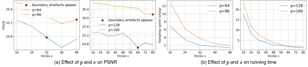
Fig. 4: Analysis of p and s on enhancing efficiency and effectiveness. Results are obtained by running on the LOL-v2-Real testing set. The red dot indicates the minimum s at which patch boundary artefacts become noticeable. (a) We notice that the patch size can affect enhancement quality. Larger patch sizes are robust to different strides without severe performance drops. (b) Using larger strides can significantly reduce running time.
