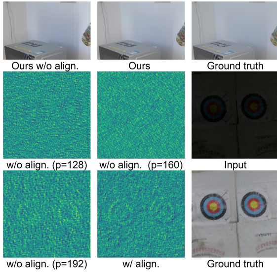
Fig. 10: Effects of the multi-patch alignment at the image level (top row) and feature level (bottom two rows).
