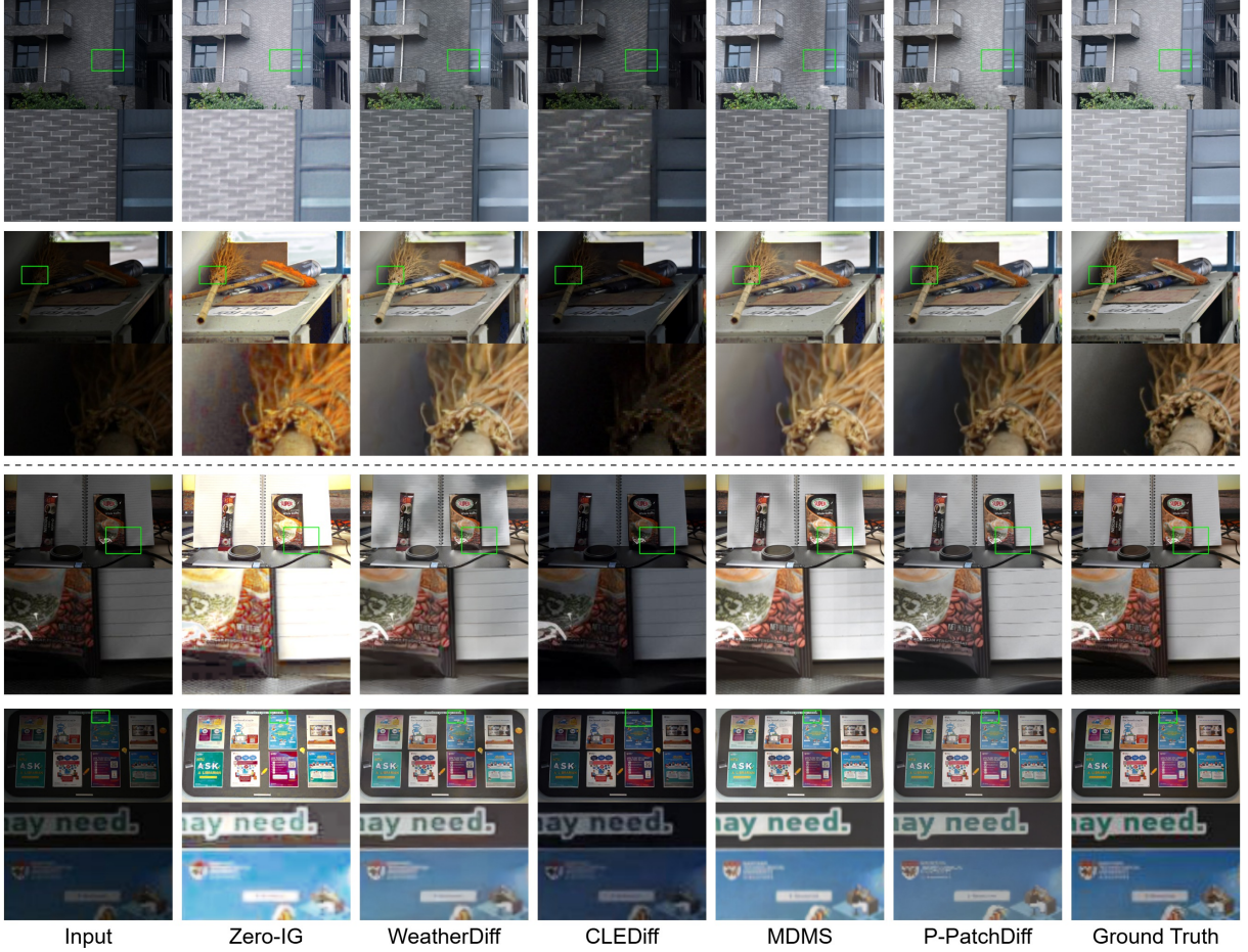
Fig. 8: Qualitative comparison on the LSRW (above the dashed line) and UHD-LL (below the dashed line).
