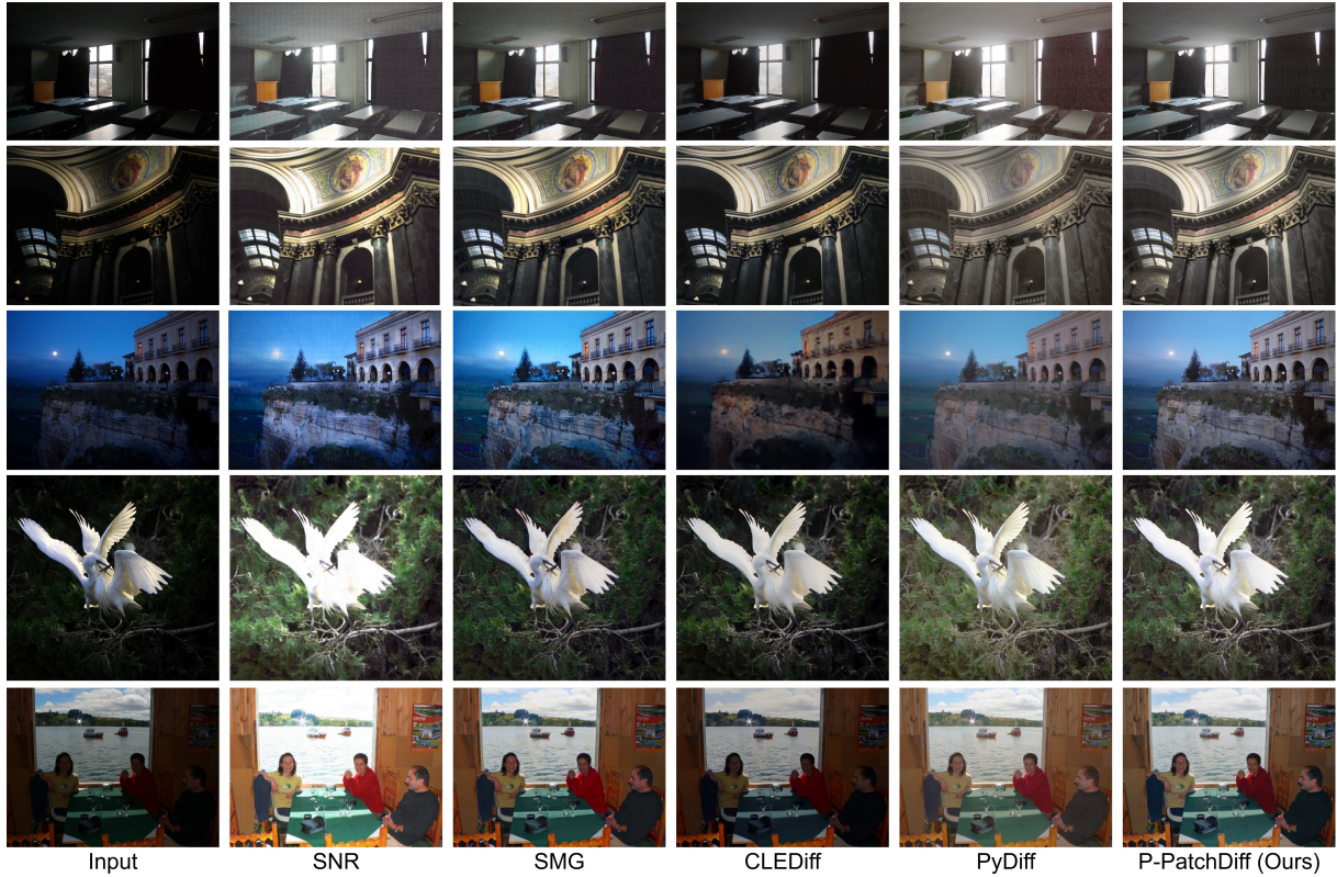
Fig. 9: Visual results on the DICM, MEF, LIME, NPE and VV datasets (From top to bottom).
