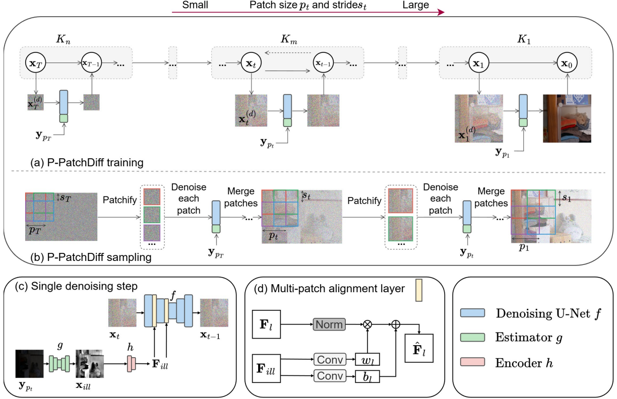
Fig. 6: Overall framework of P-PatchDiff. We divide the total time steps T into n equal-length subsets K . (a) During training, we randomly crop a patch \mathbf{x}_t^{(i)} with size p_t , where 1 \leq t \leq T , from the normal-light image \mathbf{x}_0 for diffusion and denoising. The patch size p_t is progressively increased to capture multi-level image content. (b) During sampling, the stride s_t is also progressively increased to reduce the number of patches. (c) We downsample the low-light image to \mathbf{y}_{p_t} with a size of p_t \times p_t . An estimator g is then utilised to produce the global brightness proxy \mathbf{x}_{ill} , which is subsequently processed by the encoder h to extract \mathbf{F}_{ill} . (d) The structure of the multi-patch alignment layer in f . We utilise \mathbf{F}_{ill} to normalise the encoder feature \mathbf{F}_l and generate the enhanced features \hat{\mathbf{F}}_l .
