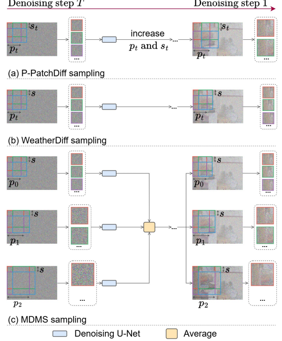
Fig. 3: Comparison of sampling strategy between WeatherDiff (Özdenizci and Legenstein 2023), MDMS (Shang et al. 2024) and our P-PatchDiff. (a) We incorporate multi-level information by increasing patch sizes. We also use larger strides for larger patch sizes to reduce the number of patches since the large patches are robust to changes in strides. (b) WeatherDiff lacks multi-level information since it only uses a fixed patch size. (c) MDMS incorporates multi-level information by creating multiple copies of the same noisy image and cropping each copy with a different patch size, thereby incurring substantial computational costs.
