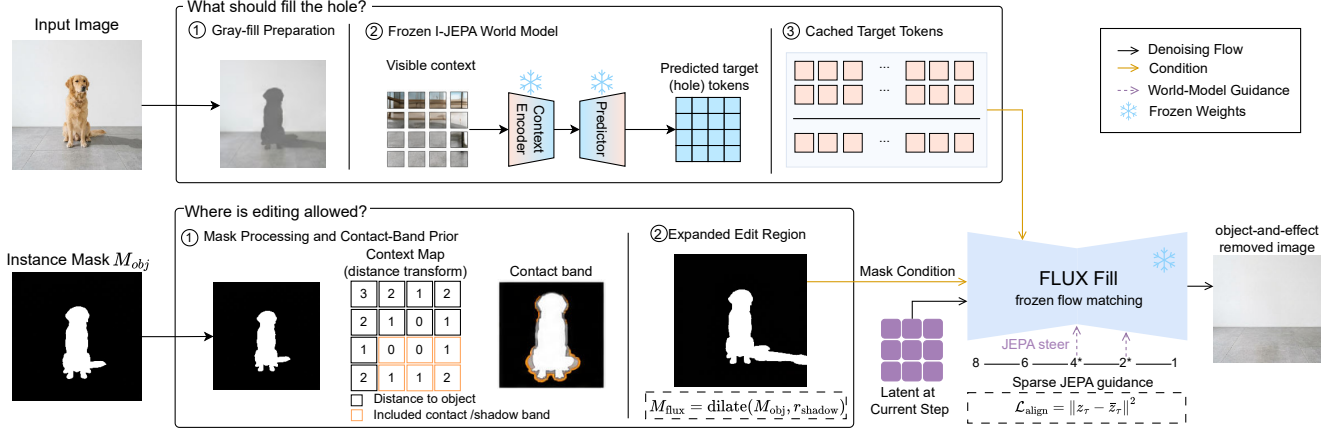
Figure 2. PredErase training-free pipeline. Top : gray-filled I_{\text{vis}} lets frozen I-JEPA predict and cache hole tokens \mathbf{E}_{\text{target}} . Bottom : a contact-band prior expands M_{\text{obj}} into the effect-aware Fill support M_{\text{flux}} . Center : frozen FLUX.2-klein-4B follows its native trajectory; at t \in \{4, 2\} , decoded features are aligned with \mathbf{E}_{\text{target}} (Eq. 8) and projected so that the additional I-JEPA update is zero outside the editable latent support (Eq. 10). No model weights are updated.
