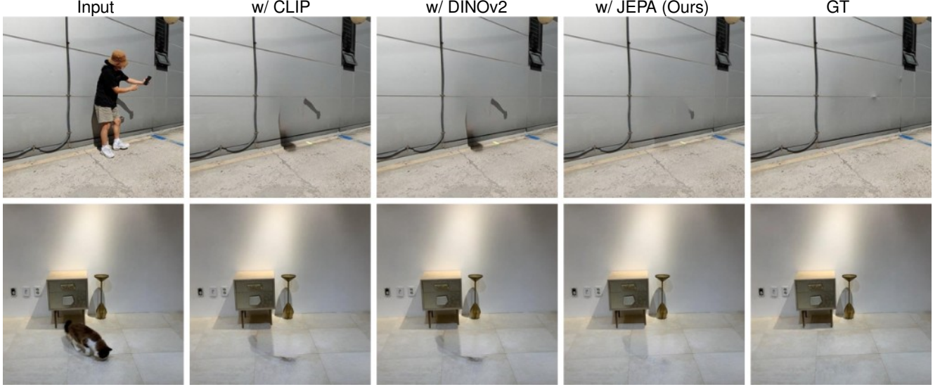
Figure 5. Qualitative guidance prior comparison under the matched Full stack (same M_{\text{flux}} , prefill, shadow-aware prompt, and sparse schedule as Table 4). Columns: Input, w/ CLIP patch, w/ DINOv2 patch, w/ JEPA (Full PredErase), and clean-plate GT. CLIP and DINOv2 remove the instance but leave dark support-plane residuals; JEPA cleans cast/contact shading closer to GT.
