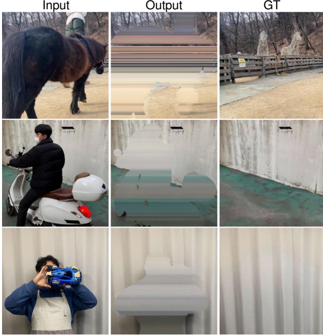
Figure 6. Failure cases on large targets (RORD-Val). Columns: Input, PredErase output, clean-plate GT. When the instance dominates the frame, visible context is thin and JEPA-guided Fill under-constrains the hole, yielding streaky or smeared silhouettes rather than coherent support reconstruction.
