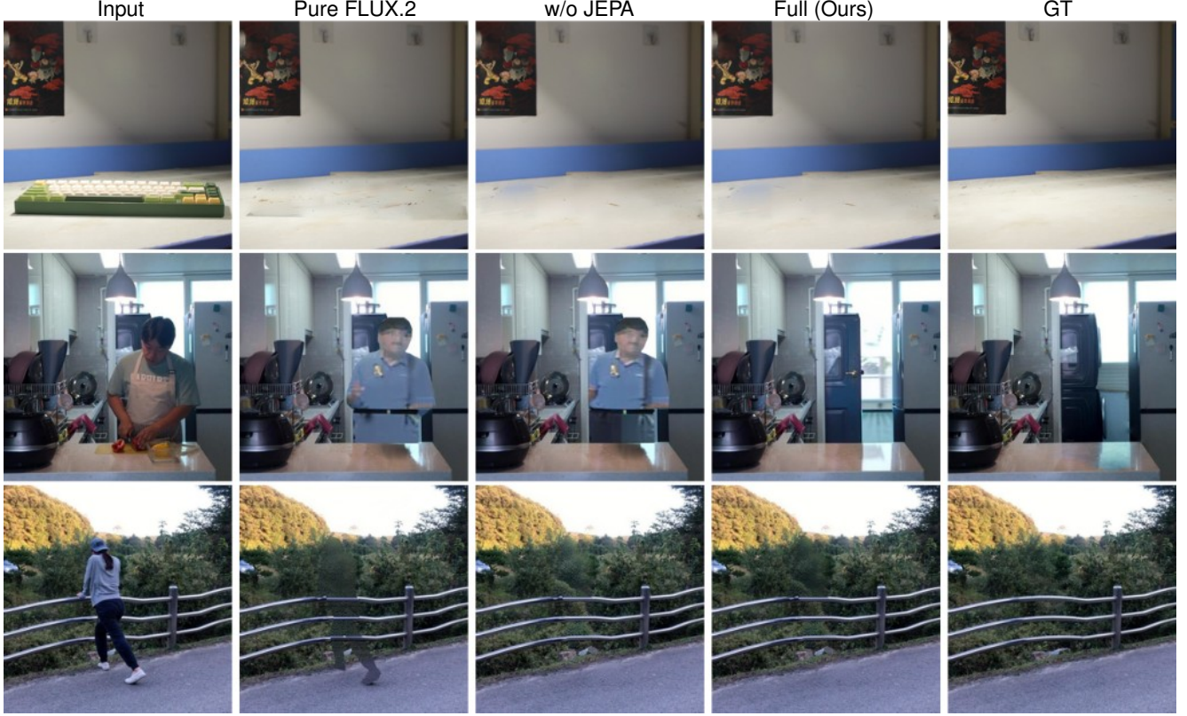
Figure 4. Qualitative module ablation under the same instance-only masks. Columns: Input, Pure FLUX.2 (native), w/o JEPA (expanded M_{\text{flux}} without feature guidance), Full PredErase, and clean-plate GT. Pure FLUX.2 leaves gray fills or ghost silhouettes; w/o JEPA improves cleanup but remains structurally incomplete; Full recovers support and background structure closer to GT.
