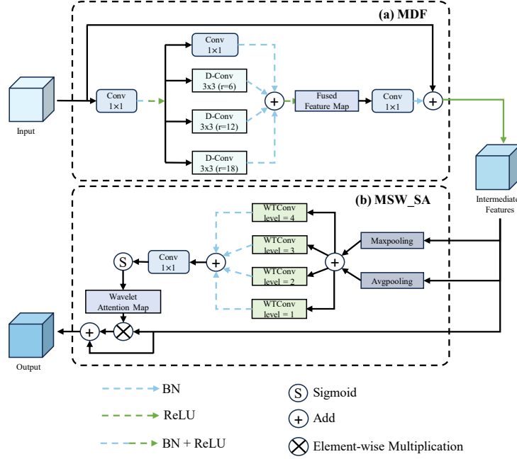
Fig. 4 The architecture of the Multi-scale Contextual Localization Module (MCLM). The module consists of two components: (a) the Multi-scale Dilation Fusion (MDF) unit, which captures multi-scale context, and (b) the Multi-Scale Wavelet Spatial Attention (MSW_SA) unit, which refines the features to localize lesion regions.
