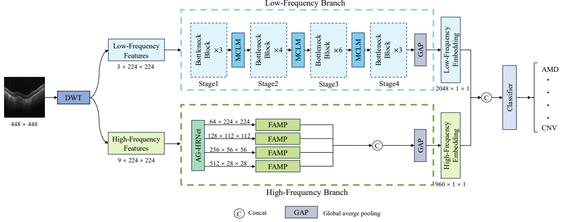
Fig. 2 The overall architecture of the proposed RetiWave-Mamba framework.
