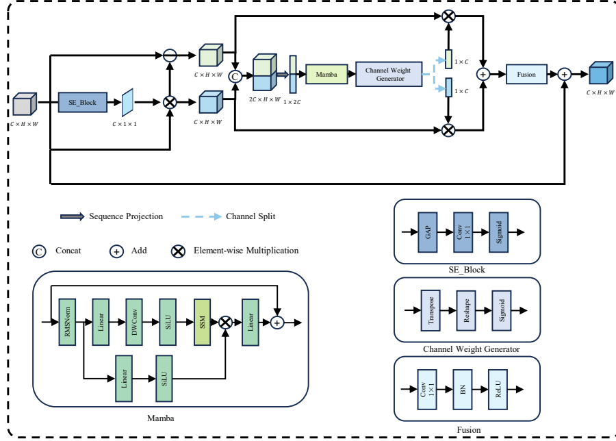
Fig. 6 The architecture of the Frequency-Adaptive Mamba Projector (FAMP). The diagram shows the main operational flow and the internal structures of its key components: the Mamba block, the SE_Block (dynamic filter), and the Fusion (convolutional) block. The main path shows an input X being split into low- and high-frequency paths by the SE_Block. The Mamba module generates adaptive channel weights ( W_L, W_H ) to re-weight these paths, which are then combined and added to the original input via a final residual connection.
