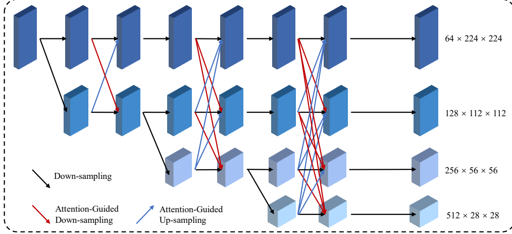
Fig. 5 The architecture of the Attention-Guided High-Resolution Network (AG-HRNet). The module operates on parallel branches. Diagram Key: Black arrows represent Standard Down-sampling for stage transitions. Red arrows represent Attention-Guided Down-sampling, and blue arrows represent Attention-Guided Up-sampling. All colored arrows indicate the use of the Attention-Guided Fusion (AGF) mechanism.
