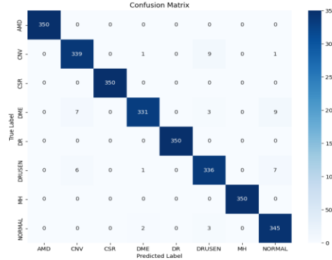
Fig. 8 The confusion matrix of the results, with an accuracy of 98.25%
