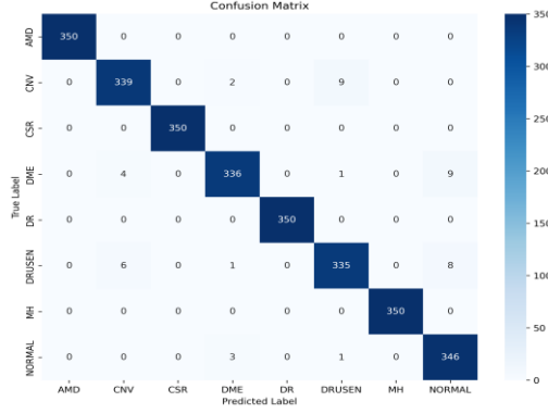
Fig. 10 Confusion matrix of the Standard Mamba
