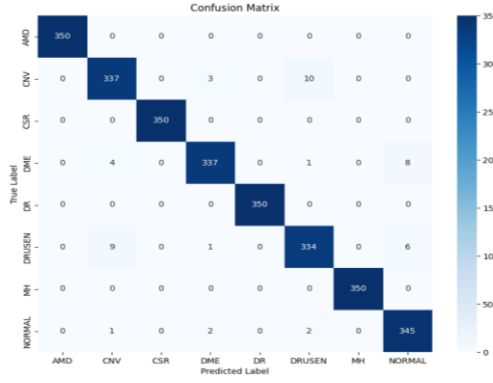
Fig. 9 Confusion matrix of the standard HRNet
