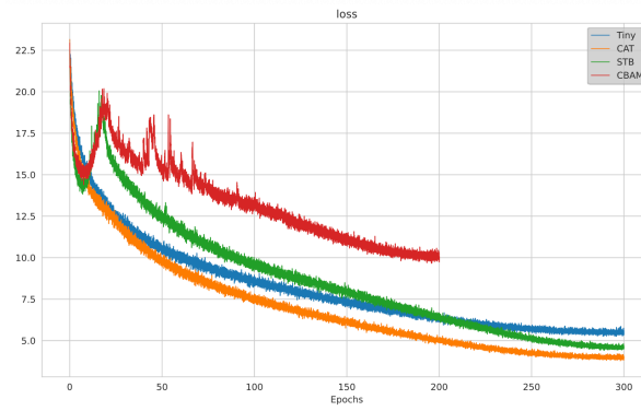
Fig. 5. Loss curve comparison
