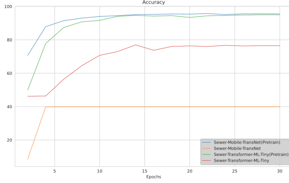
Fig. 13. Accuracy Curve Comparison (Sewer-Capsule Dataset)
