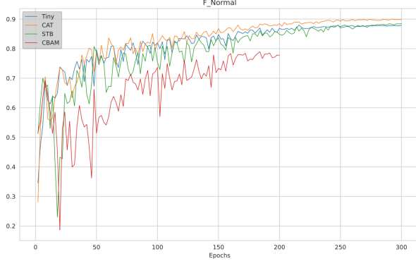
Fig. 6. F_1 Precision Curve Comparison
