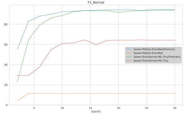
Fig. 14. F1 Accuracy Curve Comparison (Sewer-Capsule Dataset)
