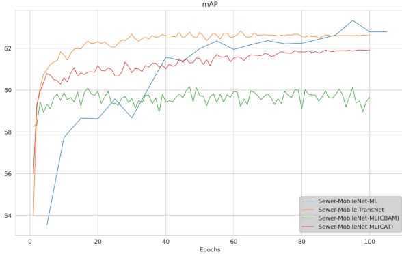
Fig. 11. mAP accuracy curve comparison
