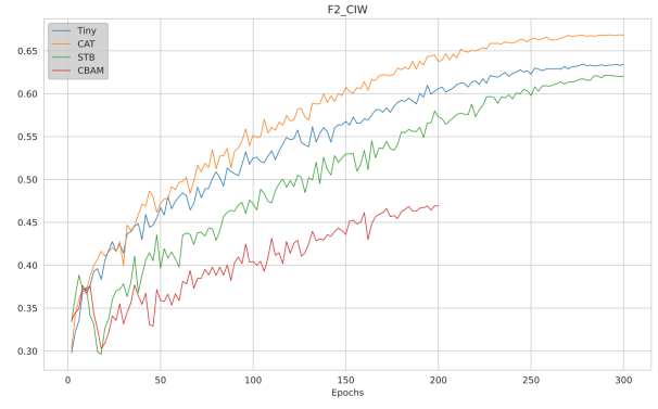
Fig. 7. F2_{CIW} Accuracy Curve Comparison
