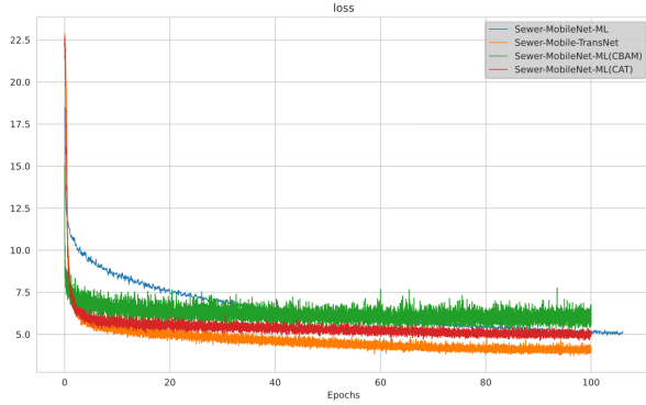
Fig. 9. Loss Curve Comparison
