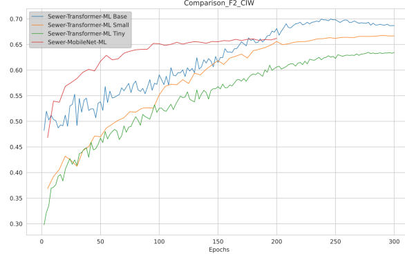
Fig. 4. F2_{CIW} Accuracy Curve Comparison
