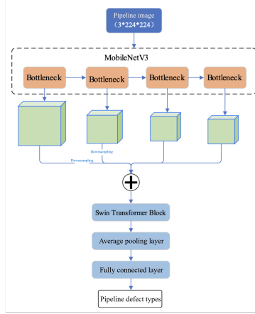
Fig. 3. Sewer-Mobile-TransNet for sewer defect classification based on a lightweight network and multi-head shifted-window self-attention
