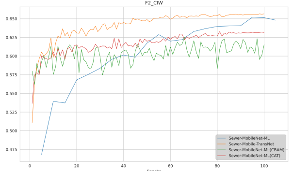
Fig. 12. F2_{CIW} Accuracy Curve Comparison
