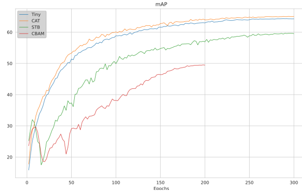
Fig. 8. mAP accuracy curve comparison
