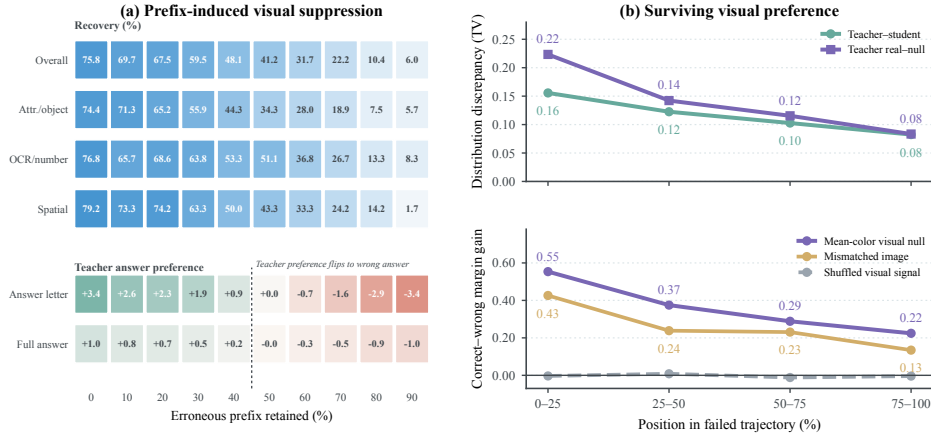
Figure 1: Erroneous prefixes mask privileged visual supervision. (a) As failed reasoning accumulates, the teacher’s preference flips from the correct to the wrong answer. (b) The teacher–student discrepancy collapses, yet an intra-teacher visual contrast retains a strong preference for the correct answer. Token shuffling destroys this signal, confirming a token-specific visual preference.
