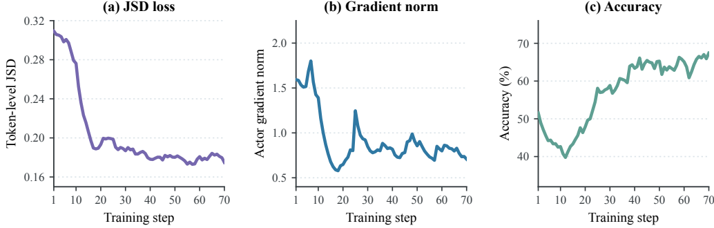
Figure 9: Training dynamics of the 4B student with \beta = 4 . (a) Token-level JSD falls sharply early in training and then stabilizes. (b) The actor gradient norm follows the same transition before settling into a lower range. (c) Answer accuracy on the generated rollouts initially decreases and then recovers.
