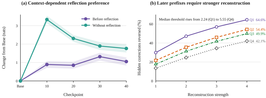
Figure 6: Context-dependent reflection and late-prefix target recovery. (a) During training, the increase in reflection-token preference recedes at positions without reflection but remains elevated immediately before reflection. (b) Stronger reconstruction reverses more wrong teacher preferences, although later prefix quartiles require greater strength.
