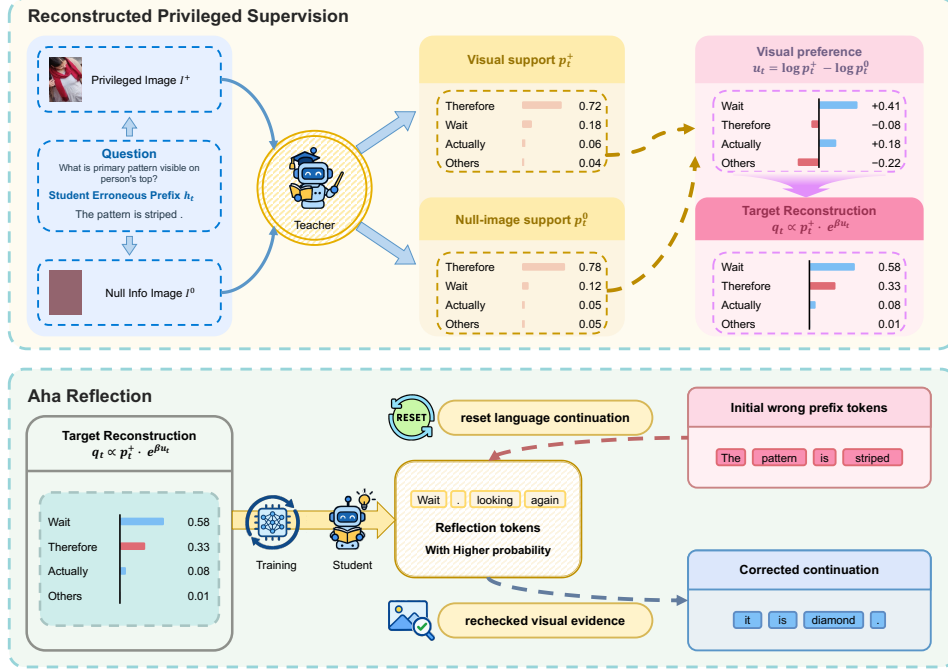
Figure 2: Overview of the OPD-Aha framework.
