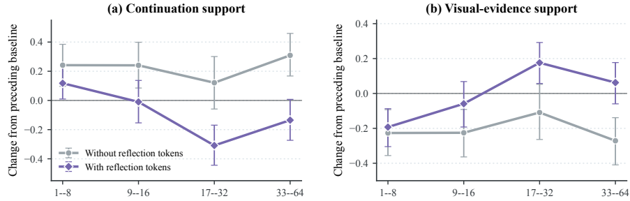
Figure 5: Visual reliance after reflection. (a) Support from the accumulated student prefix decreases after reflection. (b) Support gained from visual evidence rises after a short delay.
