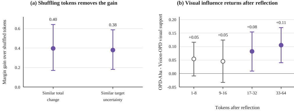
Figure 7: Token-specific correction and renewed visual support. (a) The visual preference signal produces a larger correct-option margin than token-shuffled alternatives with comparable target change or uncertainty. (b) After reflection, OPD-Aha gains more visual support for its generated tokens than Vision-OPD.
