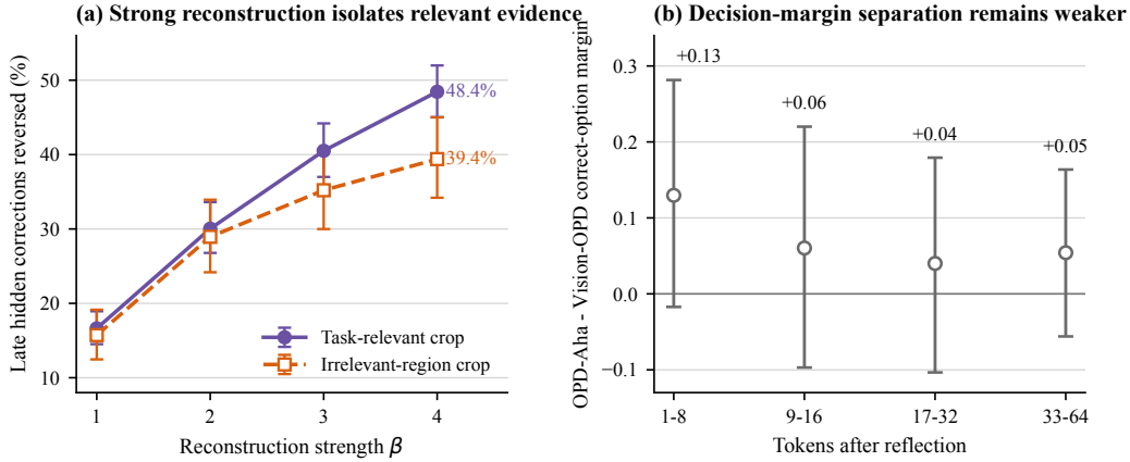
Figure 8: Evidence specificity and answer-margin dynamics after reflection. (a) As reconstruction strengthens, the task-relevant crop reverses more late wrong preferences than a same-shaped, non-overlapping crop from the same image. (b) At the same reflection prefixes, OPD-Aha maintains a larger correct-option margin than Vision-OPD.
