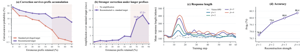
Figure 3: Late-prefix target recovery and training trends. (a, b) As hallucinated text accumulates, standard privileged distillation abandons the correct answer, whereas target reconstruction isolates the surviving visual preference to selectively amplify the correct token. (c, d) Stronger reconstruction induces a larger transient increase in response length before stabilizing, ultimately yielding consistent improvements in final accuracy.
