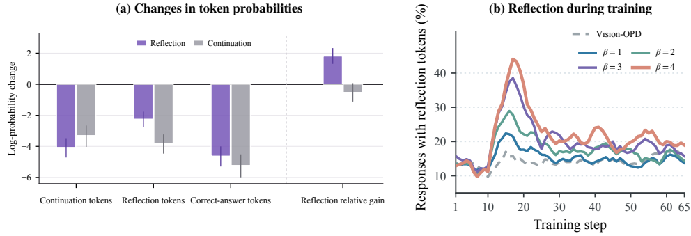
Figure 4: Token probabilities and reflection during training. (a) Target reconstruction selectively suppresses erroneous continuations before reflection, granting reflection tokens a relative advantage absent at non-reflection positions. (b) Stronger reconstruction increases the frequency of reflection tokens during training before stabilizing.
