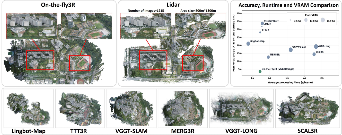
Fig. 1: Visual reconstruction results on the GauU-Scenes SZIT scene.
