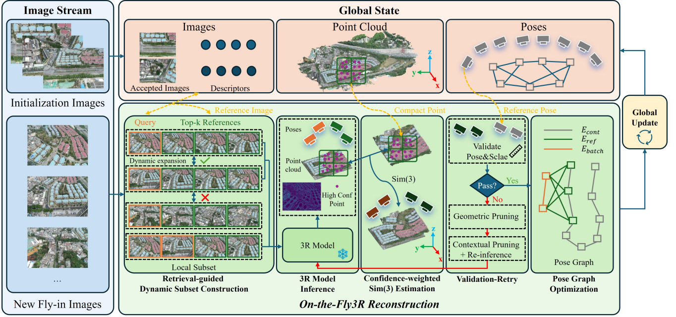
Fig. 2: Overview of the proposed On-the-Fly3R framework.
