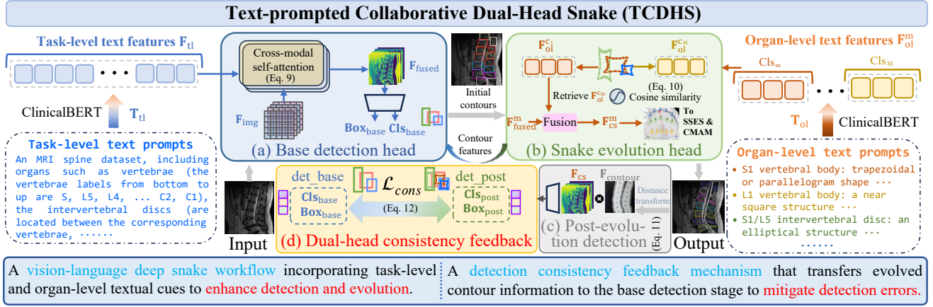
Fig. 7: The Text-prompted Collaborative Dual-Head Snake (TCDHS). In Fig. 7(a), task-level text prompts are fused with multi-scale visual features to condition the base detection head, which predicts Box_{base} , Cls_{base} , and initializes P_0 . In Fig. 7(b), organ-level text prompts are aligned with RoI features to form multi-modal feature maps F_{cs}^m for snake evolution. In Fig. 7(c), the evolved contours P are converted into contour-aware heatmaps to augment features for a post-evolution detector. In Fig. 7(d), a dual-head detection consistency loss is designed to align \{Box_{base}, Cls_{base}\} with \{Box_{post}, Cls_{post}\} , transferring the contour information to the base detector.
