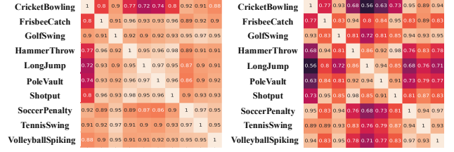
(a) w/ foreground & background (b) w/ foreground only Figure 2. Cosine similarity heatmap of the visual-aware text features produced by the cross-modal adaptation in Ti-FAD [13] across various action classes on THUMOS14 [8]. (a) With video features including both foreground and background regions, and (b) with only foreground regions used for cross-modal adaptation.
