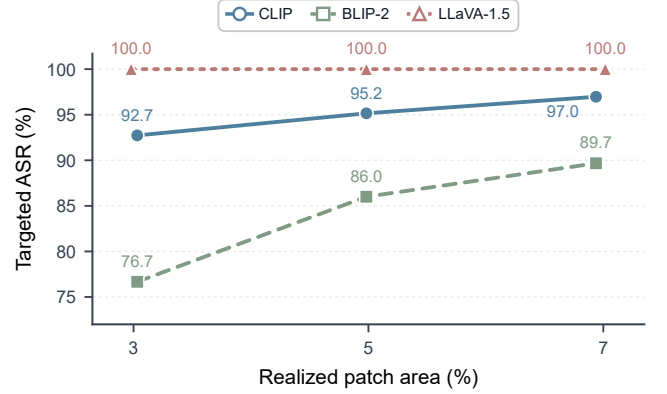
Figure 4: Targeted ASR as a function of realized patch area for the representative classification, conditional-generation, and binary-VQA variants.
