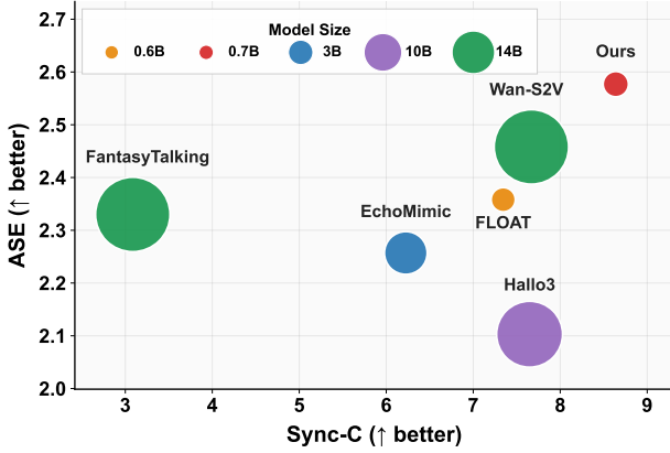
Figure 2: Comparison of recent talking avatar methods on ASE [53] and Sync-C [9]. Existing methods still struggle to jointly improve aesthetic quality and lip synchronization.
