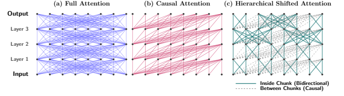
Figure 4: Comparison of audio context modeling schemes. (a) Full Attention captures global context but incurs high cost and leaks future information. (b) Causal Attention preserves causality but weakens local bidirectional interaction. (c) Our Hierarchical Shifted Attention supports bidirectional interaction within chunks and causal aggregation across chunks, while progressively enlarging the receptive field.
