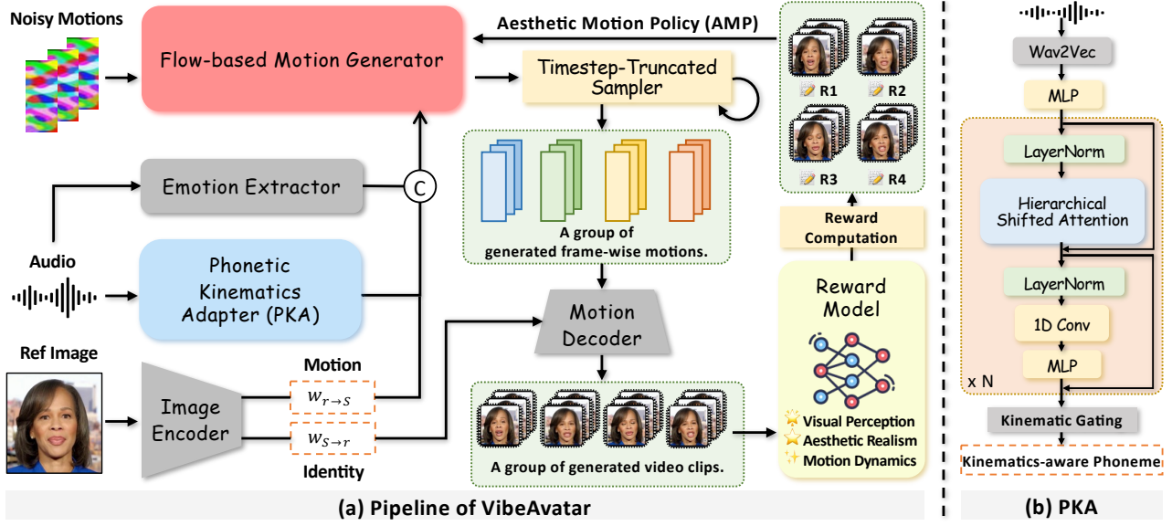
Figure 3: Overview of VibeAvatar. (a) The framework integrates a lightweight flow-based motion generator, a Phonetic Kinematics Adapter (PKA), and an Aesthetic Motion Policy (AMP) to improve lip articulation, motion aesthetics, and inference efficiency. (b) PKA transforms generic speech features into phonetic-kinematic conditions through hierarchical shifted attention, enabling local bidirectional interaction, causal aggregation, and a progressively enlarged receptive field for accurate lip articulation.
