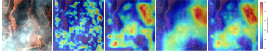
Figure 2: Multi-layer Grad-CAM activation maps produced by the teacher model trained with tile-level supervision. Grad-CAM maps from Layers 2–4 and their fused result illustrate the emergence of spatial attention from classification-only training.
