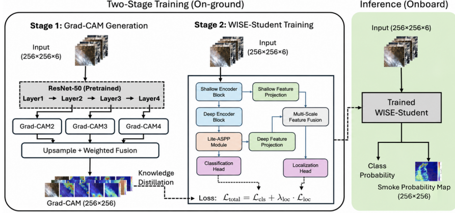
Figure 1: Overall WISE pipeline. A teacher model generates Grad-CAM attention maps, which guide training of the lightweight WISE-Student for joint smoke detection and localization during onboard inference.
